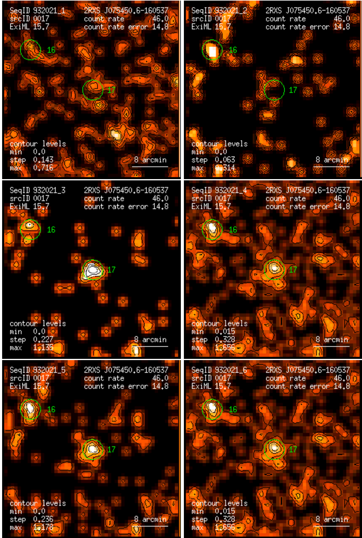
Figure 17: RASS 932021: detection 0017: band rate images, Gaussian filter: (1) PSPC channels 11 – 41, (2) 52 – 90, (3) 91 – 201, (4) 11 – 235, (5) 52 – 201, (6) 11 – 201. Broad band rates in counts/ks. Band rate contour levels in counts/ks/arcmin 2 .
