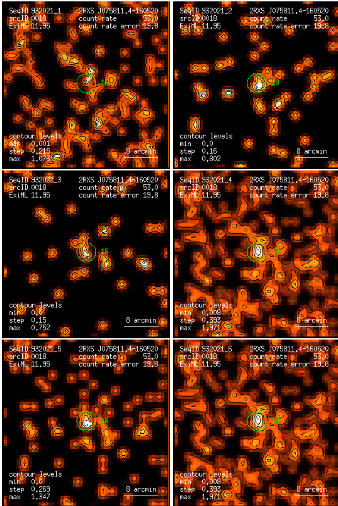
Figure 18: RASS 932021: detection 0018: band rate images, Gaussian filter: (1) PSPC channels 11 – 41, (2) 52 – 90, (3) 91 – 201, (4) 11 – 235, (5) 52 – 201, (6) 11 – 201. Broad band rates in counts/ks. Band rate contour levels in counts/ks/arcmin 2 .
