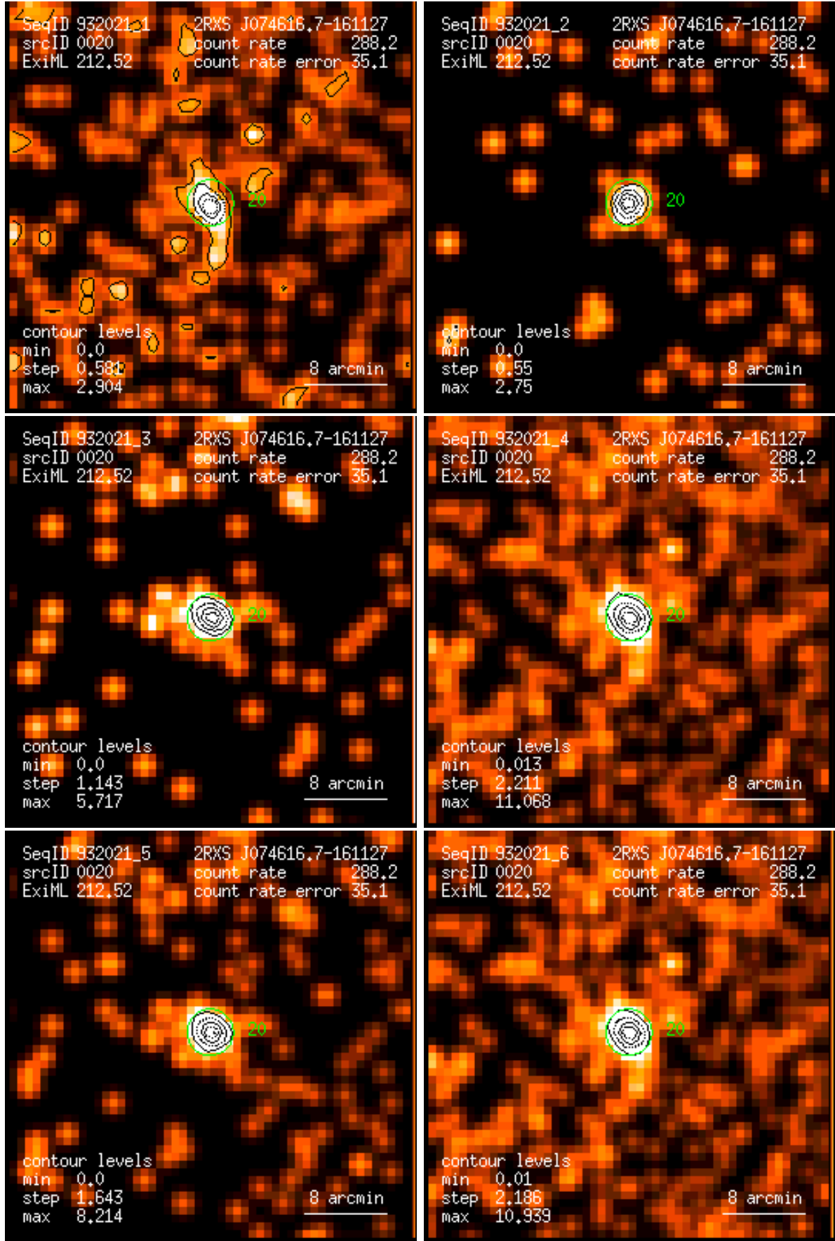
Figure 20: RASS 932021: detection 0020: band rate images, Gaussian filter: (1) PSPC channels 11 – 41, (2) 52 – 90, (3) 91 – 201, (4) 11 – 235, (5) 52 – 201, (6) 11 – 201. Broad band rates in counts/ks. Band rate contour levels in counts/ks/arcmin 2 .
