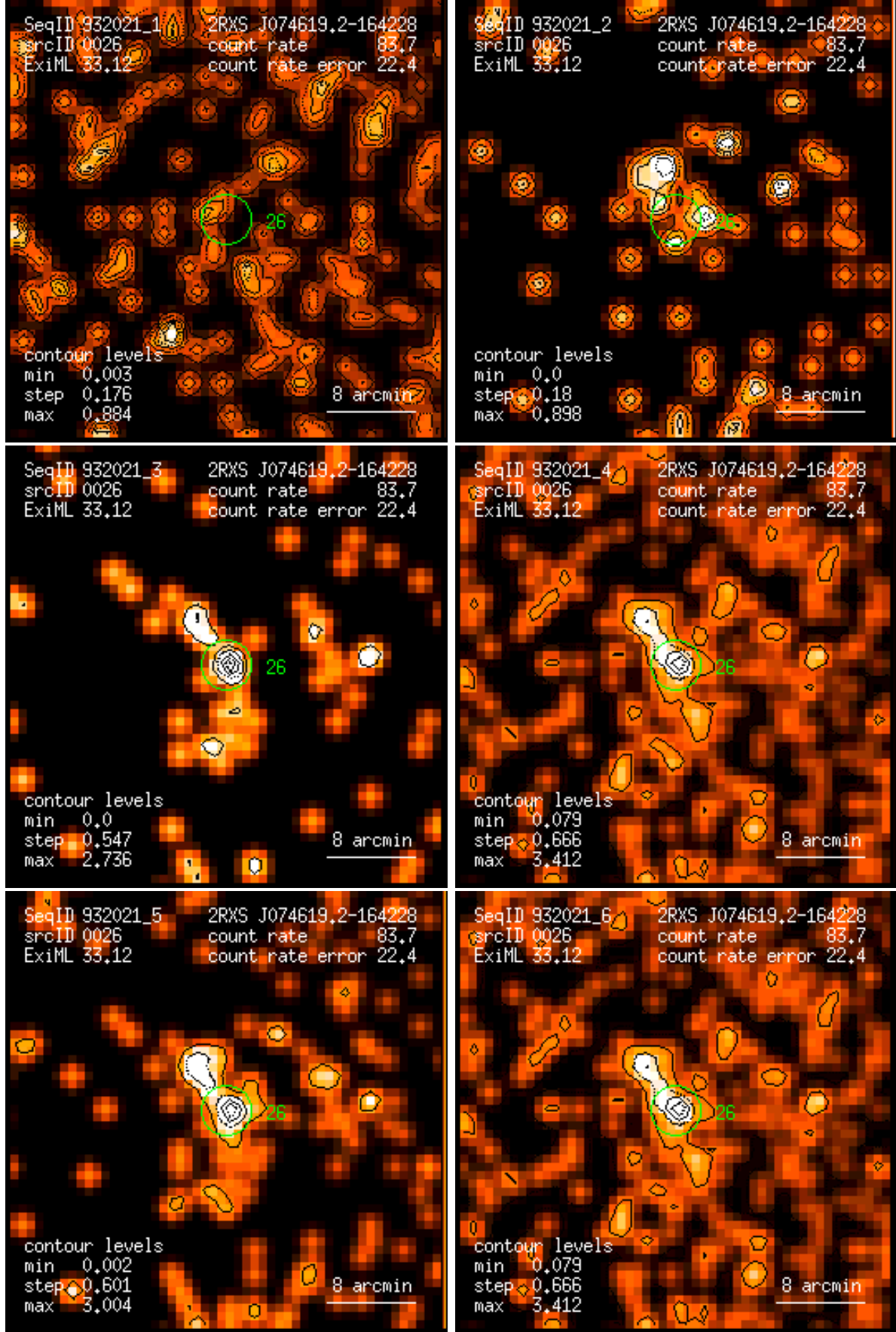
Figure 26: RASS 932021: detection 0026: band rate images, Gaussian filter: (1) PSPC channels 11 – 41, (2) 52 – 90, (3) 91 – 201, (4) 11 – 235, (5) 52 – 201, (6) 11 – 201. Broad band rates in counts/ks. Band rate contour levels in counts/ks/arcmin 2 .
