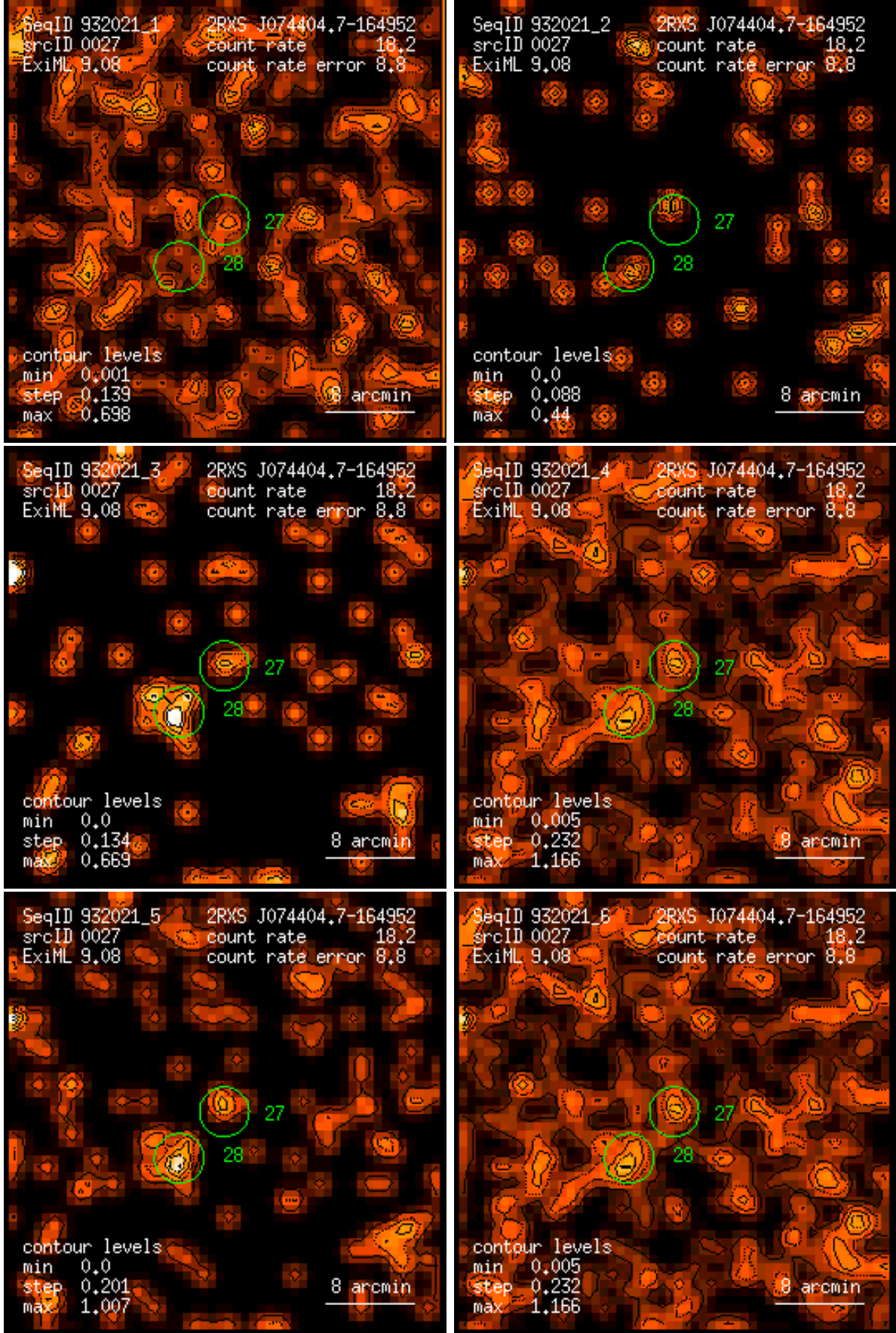
Figure 27: RASS 932021: detection 0027: band rate images, Gaussian filter: (1) PSPC channels 11 – 41, (2) 52 – 90, (3) 91 – 201, (4) 11 – 235, (5) 52 – 201, (6) 11 – 201. Broad band rates in counts/ks. Band rate contour levels in counts/ks/arcmin 2 .
