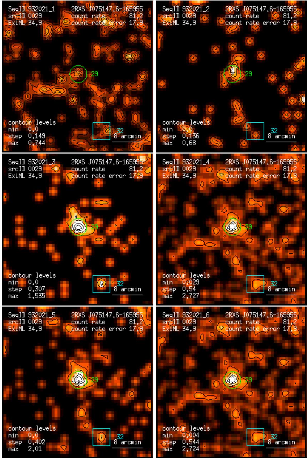
Figure 29: RASS 932021: detection 0029: band rate images, Gaussian filter: (1) PSPC channels 11 – 41, (2) 52 – 90, (3) 91 – 201, (4) 11 – 235, (5) 52 – 201, (6) 11 – 201. Broad band rates in counts/ks. Band rate contour levels in counts/ks/arcmin 2 .
