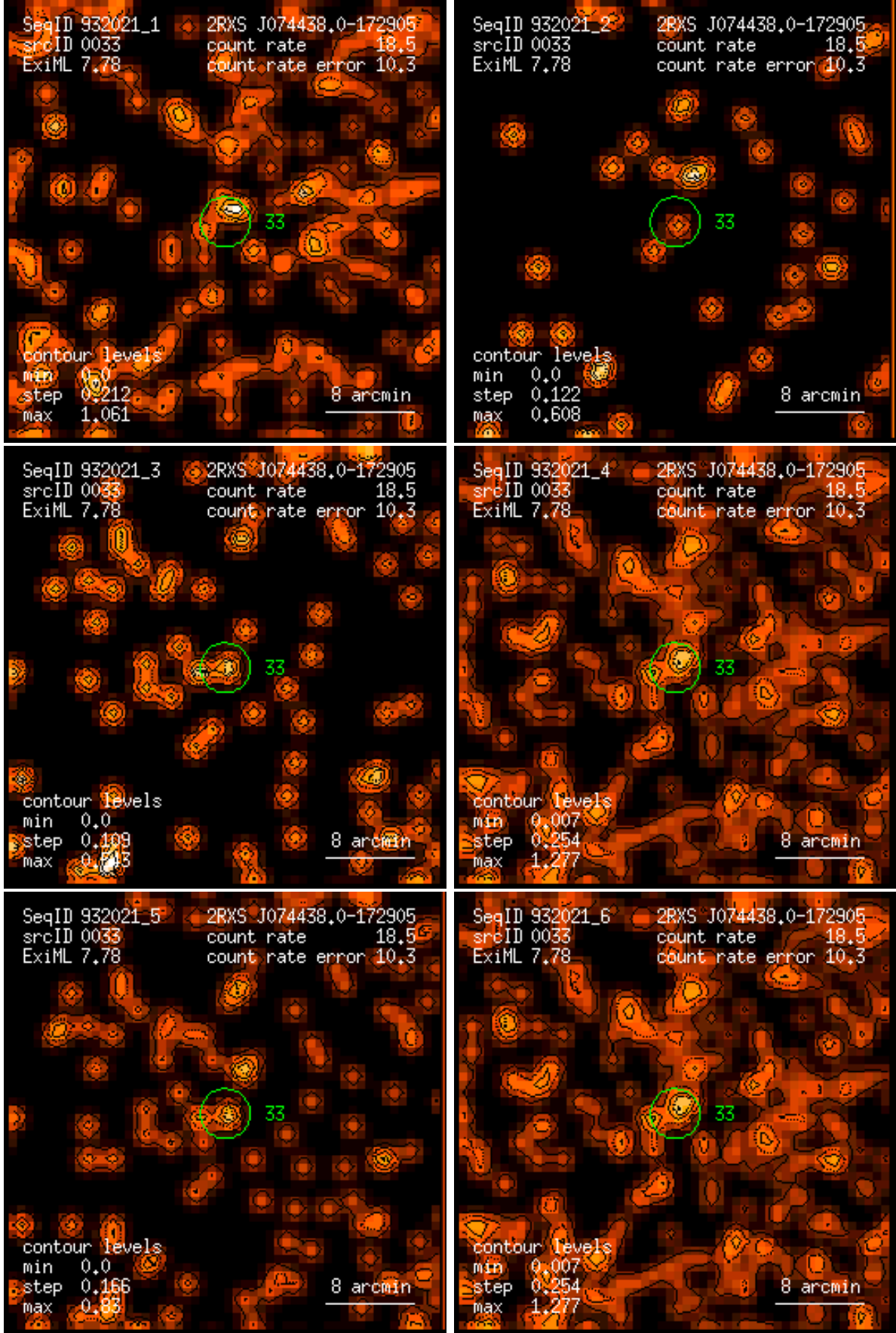
Figure 33: RASS 932021: detection 0033: band rate images, Gaussian filter: (1) PSPC channels 11 – 41, (2) 52 – 90, (3) 91 – 201, (4) 11 – 235, (5) 52 – 201, (6) 11 – 201. Broad band rates in counts/ks. Band rate contour levels in counts/ks/arcmin 2 .
