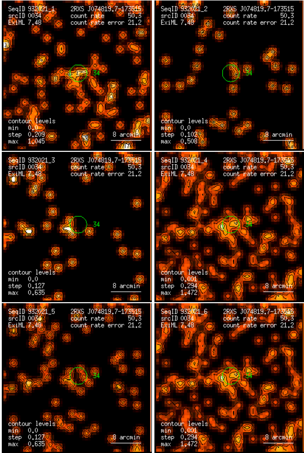
Figure 34: RASS 932021: detection 0034: band rate images, Gaussian filter: (1) PSPC channels 11 – 41, (2) 52 – 90, (3) 91 – 201, (4) 11 – 235, (5) 52 – 201, (6) 11 – 201. Broad band rates in counts/ks. Band rate contour levels in counts/ks/arcmin 2 .
