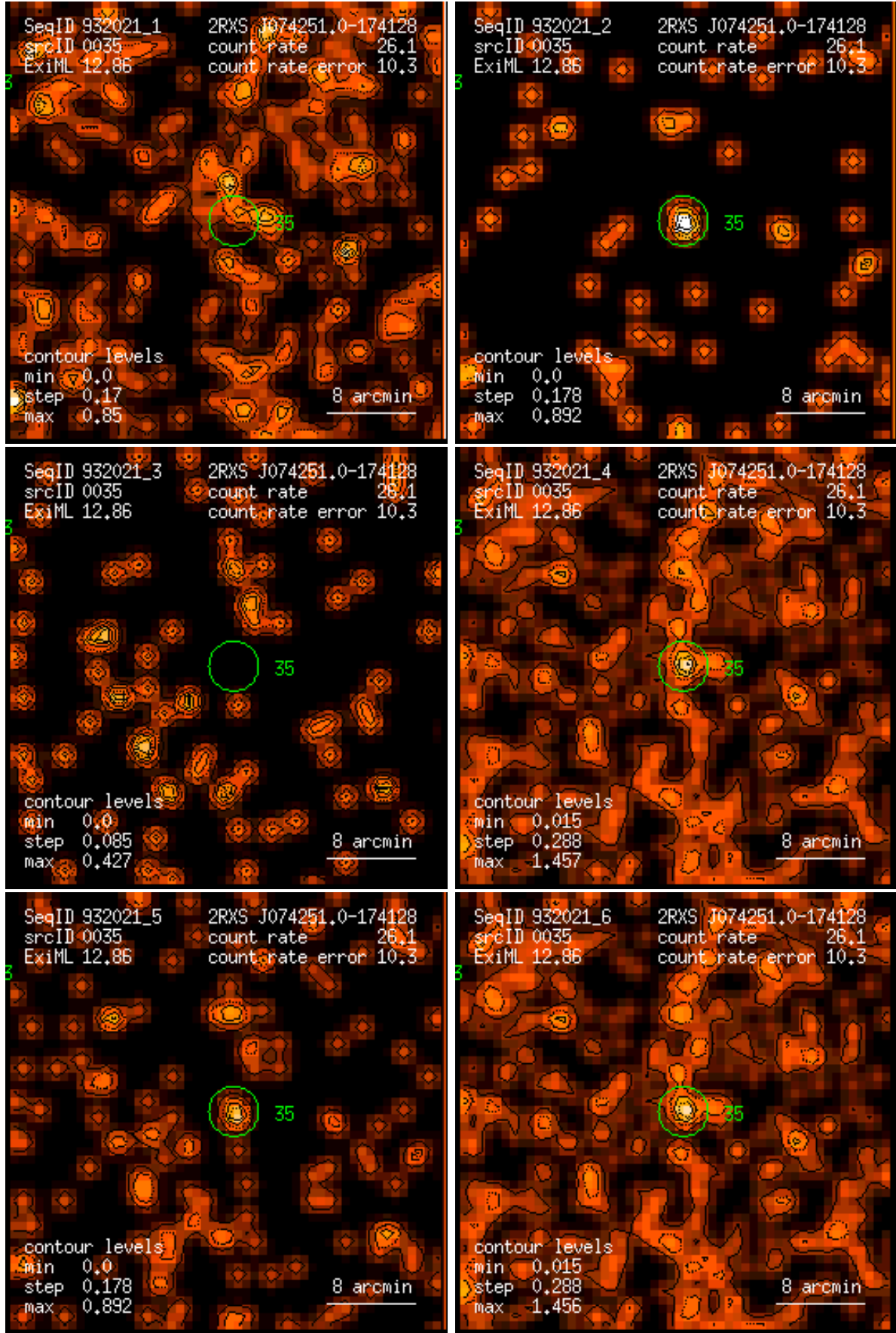
Figure 35: RASS 932021: detection 0035: band rate images, Gaussian filter: (1) PSPC channels 11 – 41, (2) 52 – 90, (3) 91 – 201, (4) 11 – 235, (5) 52 – 201, (6) 11 – 201. Broad band rates in counts/ks. Band rate contour levels in counts/ks/arcmin 2 .
