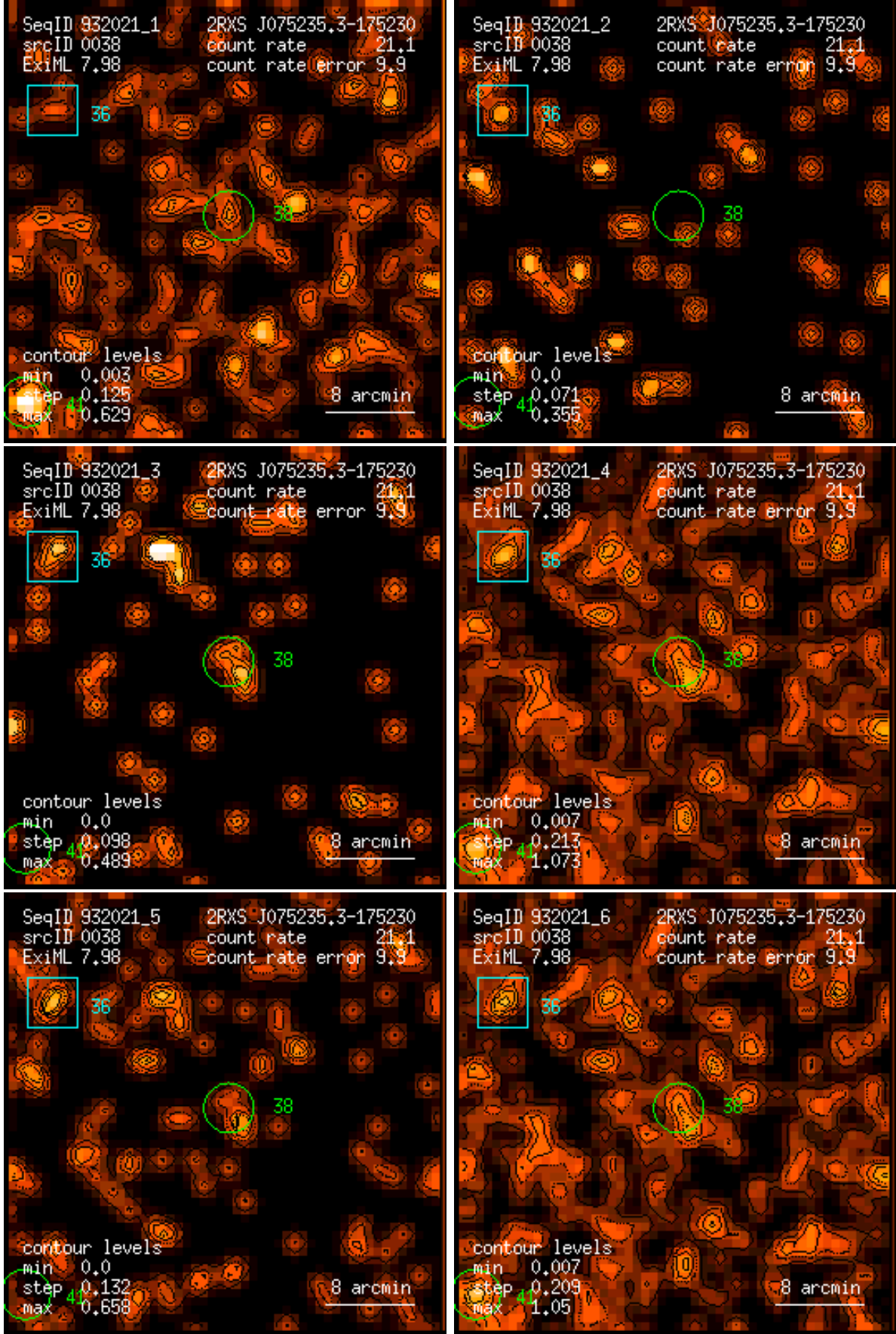
Figure 38: RASS 932021: detection 0038: band rate images, Gaussian filter: (1) PSPC channels 11 – 41, (2) 52 – 90, (3) 91 – 201, (4) 11 – 235, (5) 52 – 201, (6) 11 – 201. Broad band rates in counts/ks. Band rate contour levels in counts/ks/arcmin 2 .
