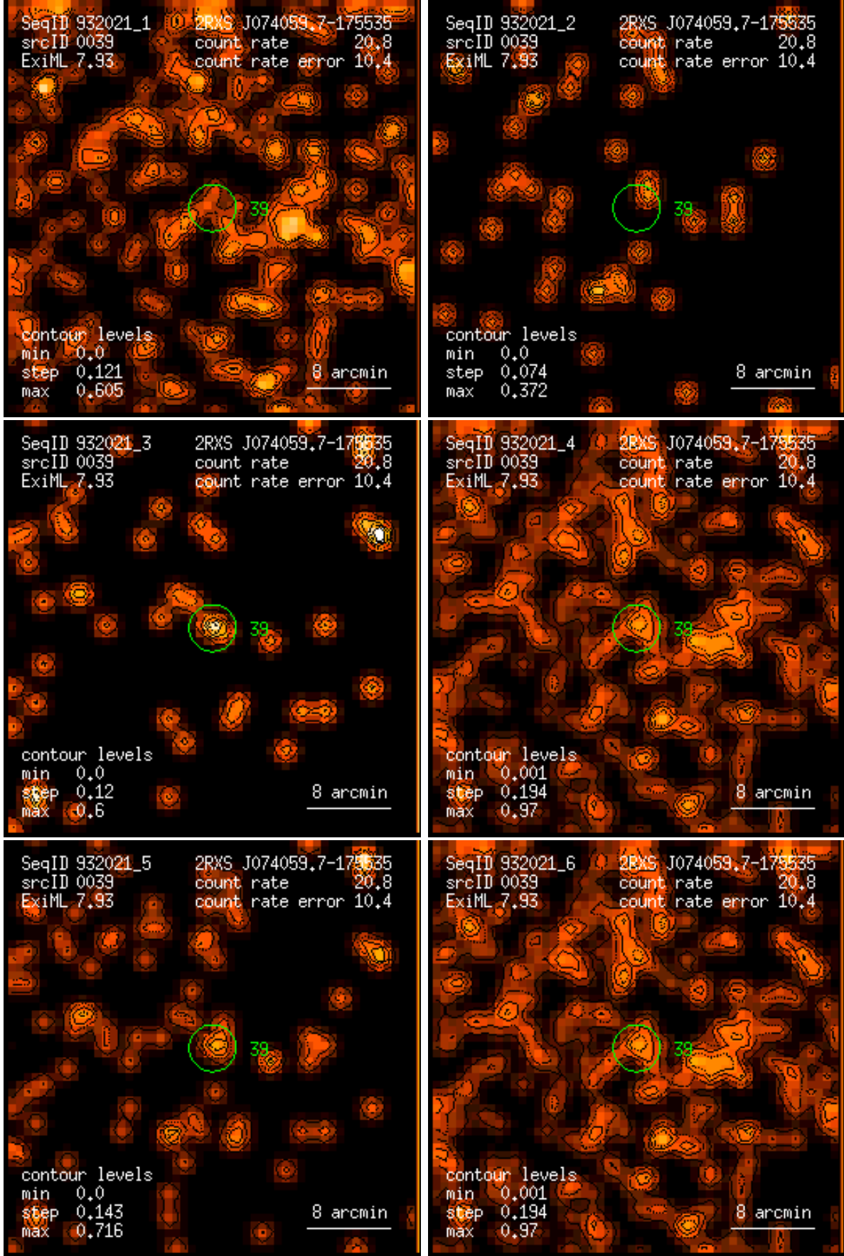
Figure 39: RASS 932021: detection 0039: band rate images, Gaussian filter: (1) PSPC channels 11 – 41, (2) 52 – 90, (3) 91 – 201, (4) 11 – 235, (5) 52 – 201, (6) 11 – 201. Broad band rates in counts/ks. Band rate contour levels in counts/ks/arcmin 2 .
