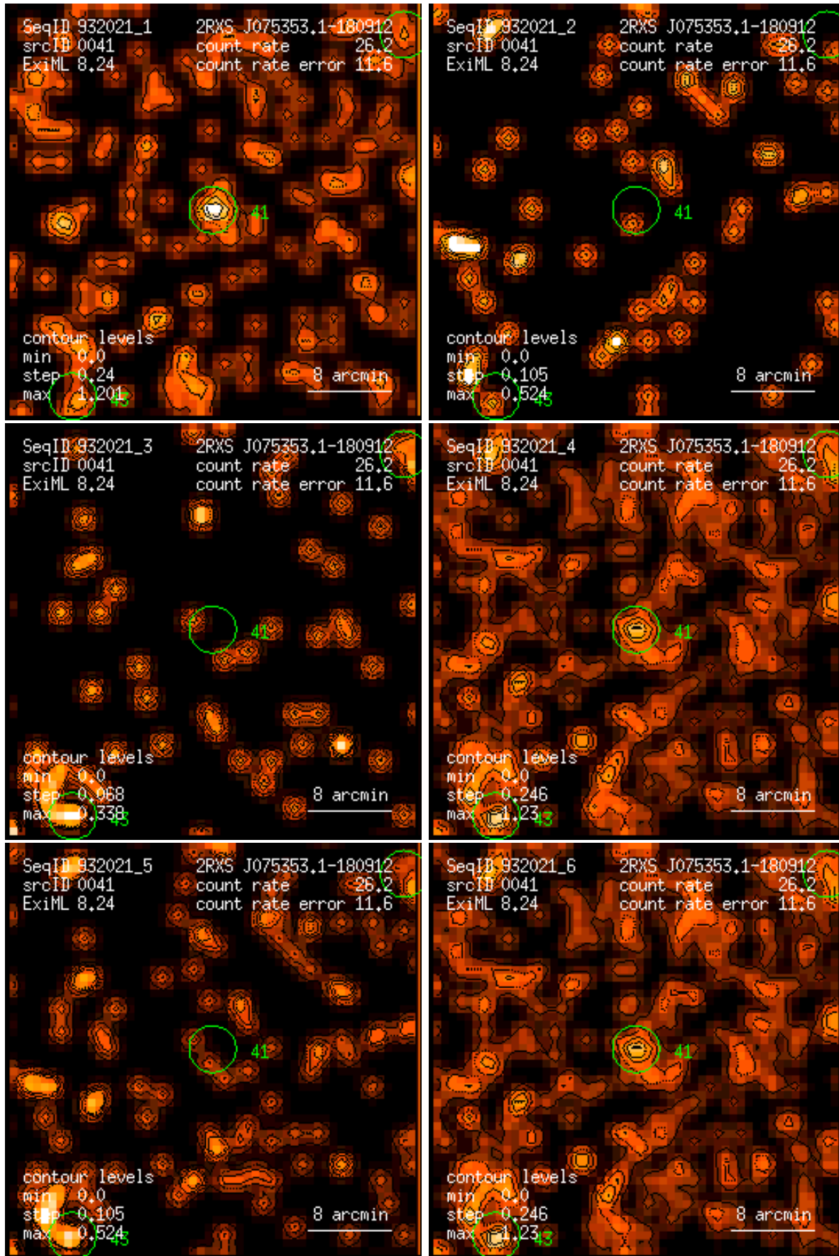
Figure 41: RASS 932021: detection 0041: band rate images, Gaussian filter: (1) PSPC channels 11 – 41, (2) 52 – 90, (3) 91 – 201, (4) 11 – 235, (5) 52 – 201, (6) 11 – 201. Broad band rates in counts/ks. Band rate contour levels in counts/ks/arcmin 2 .
