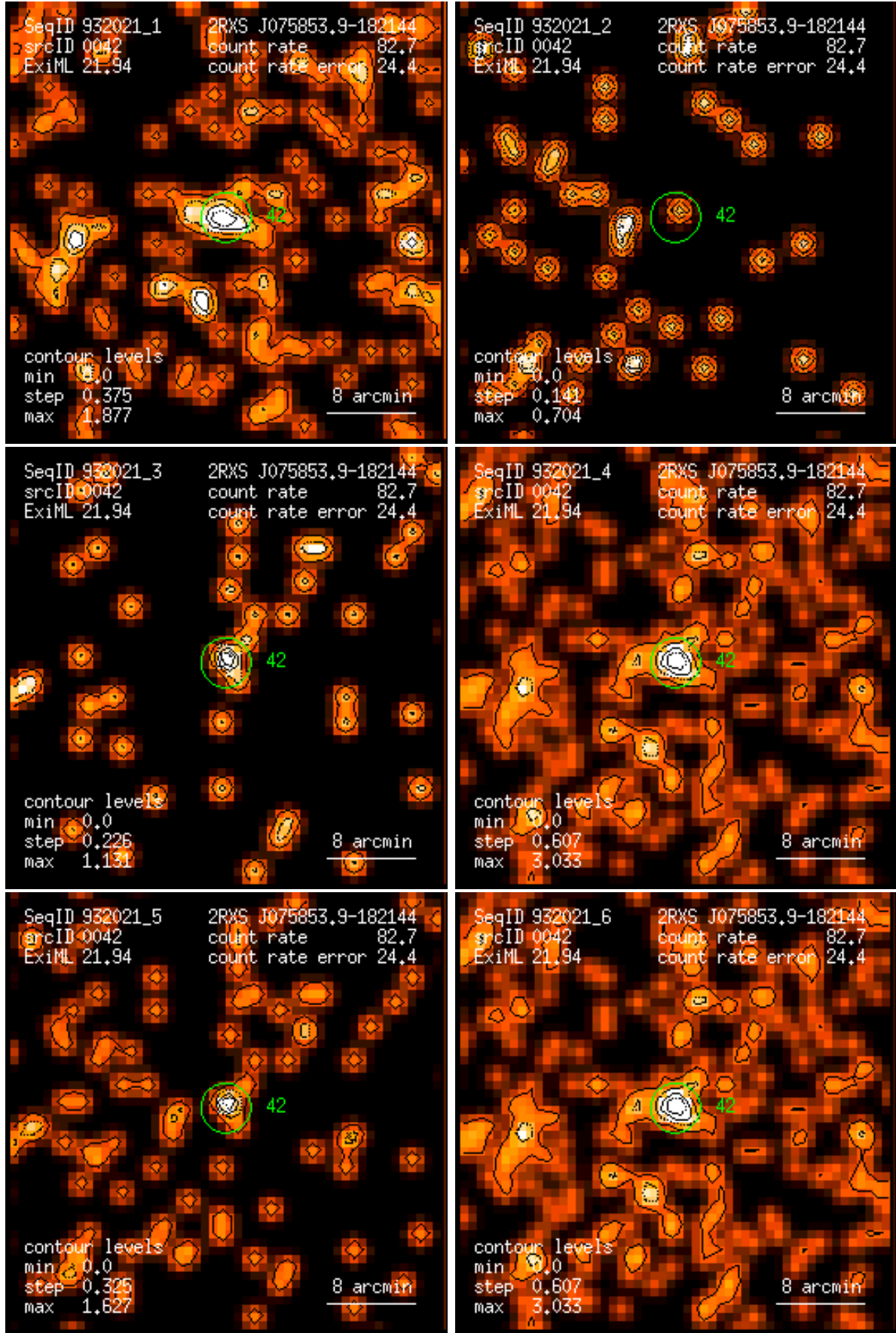
Figure 42: RASS 932021: detection 0042: band rate images, Gaussian filter: (1) PSPC channels 11 – 41, (2) 52 – 90, (3) 91 – 201, (4) 11 – 235, (5) 52 – 201, (6) 11 – 201. Broad band rates in counts/ks. Band rate contour levels in counts/ks/arcmin 2 .
