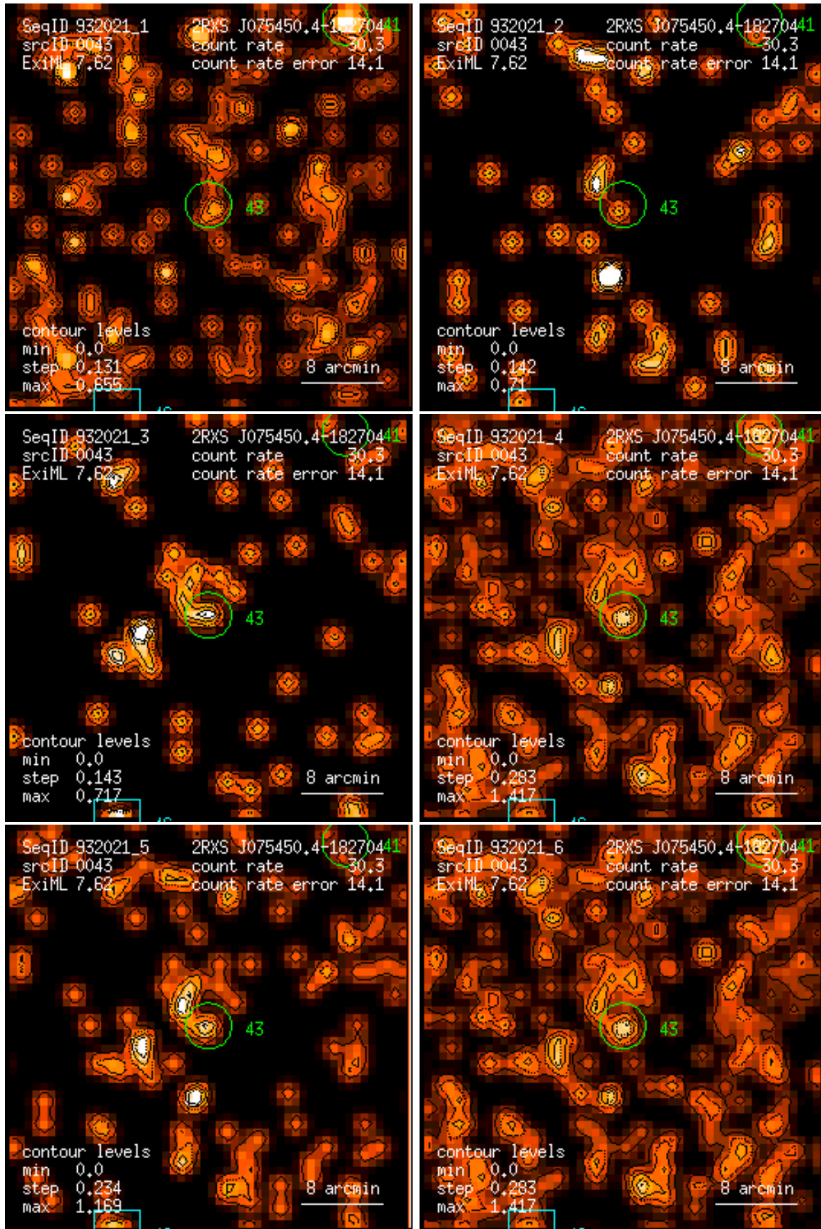
Figure 43: RASS 932021: detection 0043: band rate images, Gaussian filter: (1) PSPC channels 11 – 41, (2) 52 – 90, (3) 91 – 201, (4) 11 – 235, (5) 52 – 201, (6) 11 – 201. Broad band rates in counts/ks. Band rate contour levels in counts/ks/arcmin 2 .
