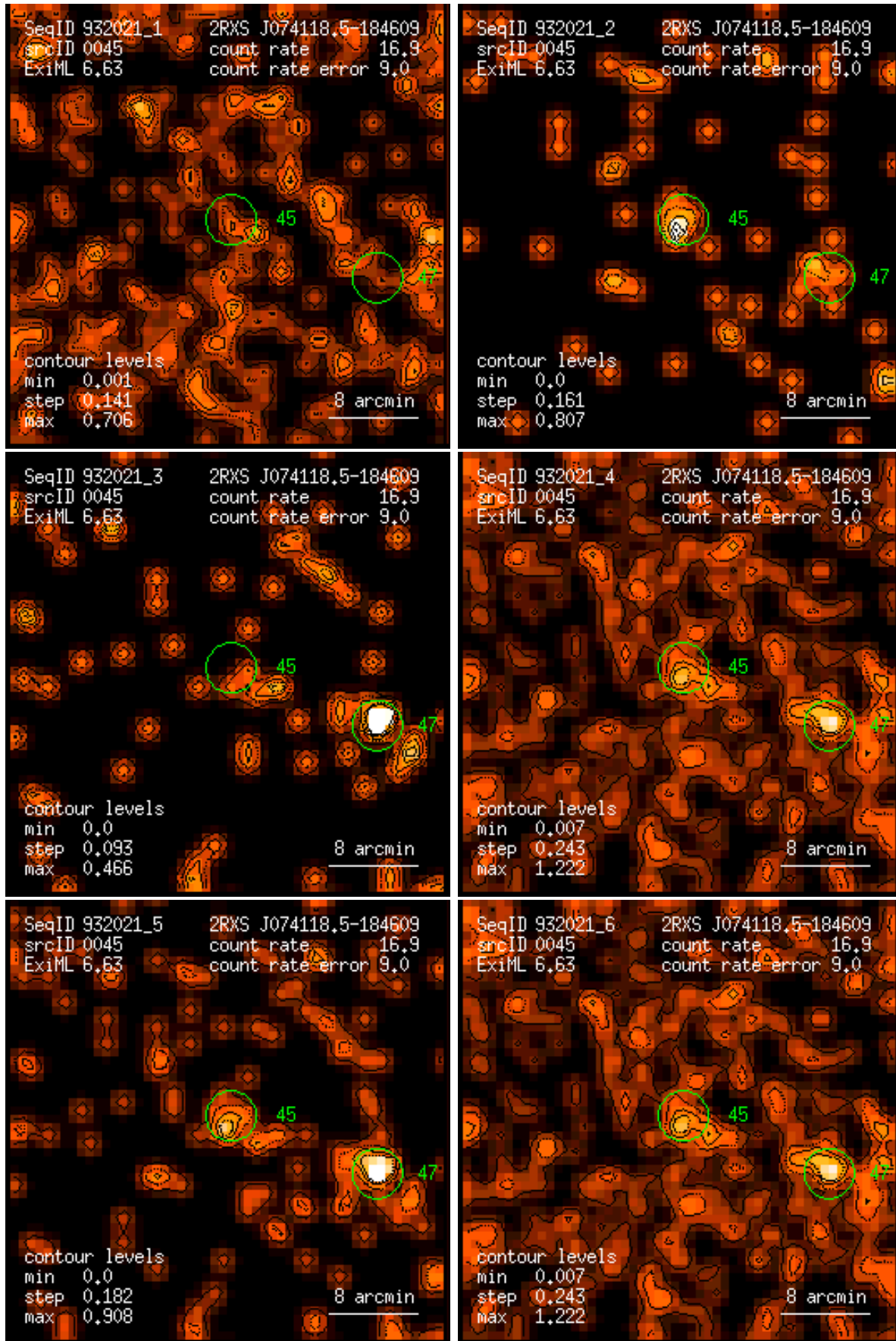
Figure 45: RASS 932021: detection 0045: band rate images, Gaussian filter: (1) PSPC channels 11 – 41, (2) 52 – 90, (3) 91 – 201, (4) 11 – 235, (5) 52 – 201, (6) 11 – 201. Broad band rates in counts/ks. Band rate contour levels in counts/ks/arcmin 2 .
