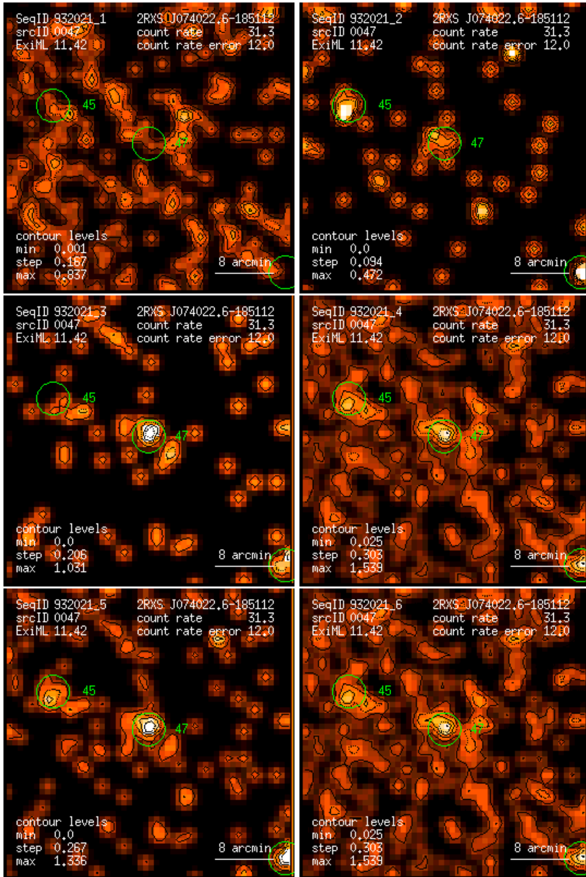
Figure 47: RASS 932021: detection 0047: band rate images, Gaussian filter: (1) PSPC channels 11 – 41, (2) 52 – 90, (3) 91 – 201, (4) 11 – 235, (5) 52 – 201, (6) 11 – 201. Broad band rates in counts/ks. Band rate contour levels in counts/ks/arcmin 2 .
