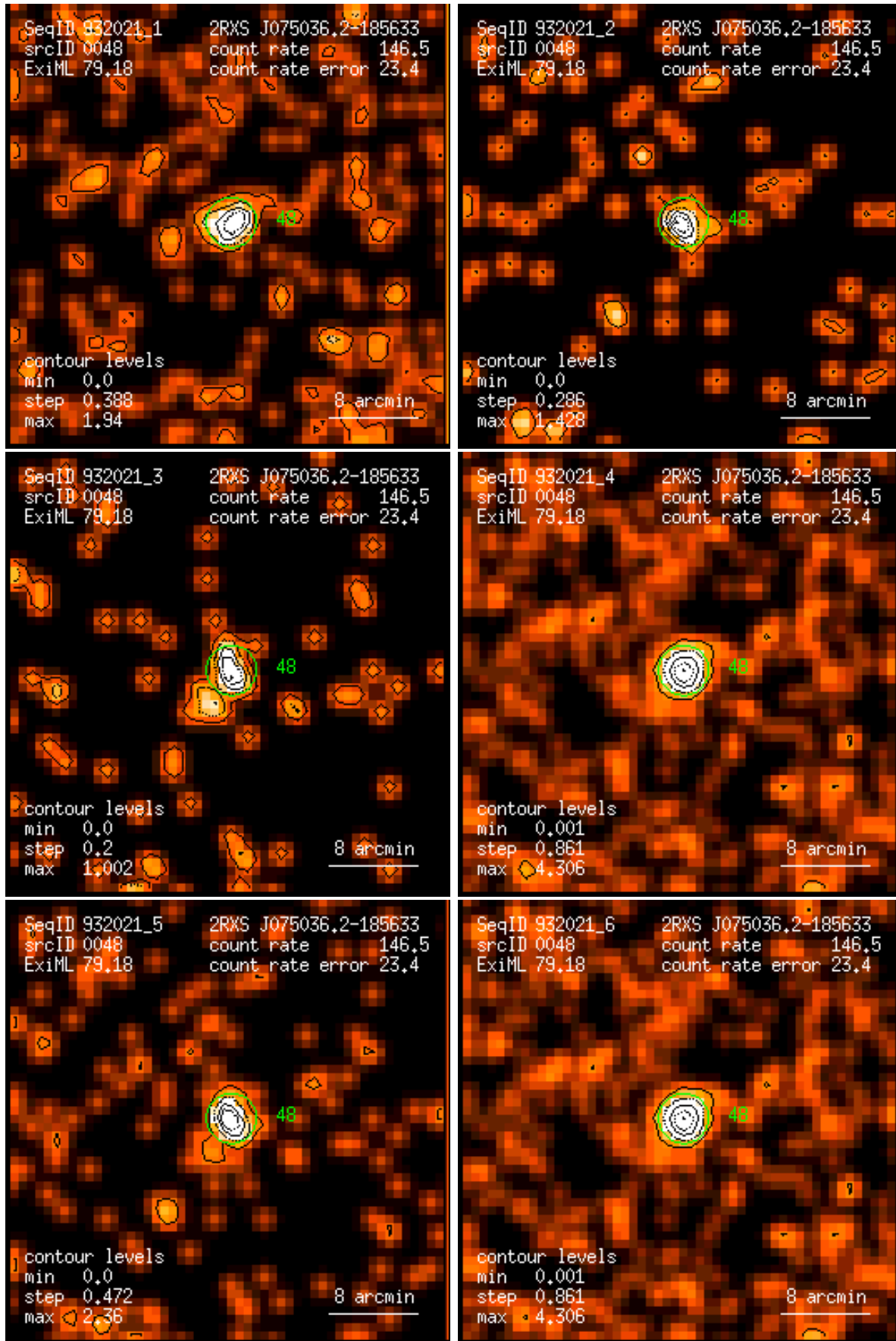
Figure 48: RASS 932021: detection 0048: band rate images, Gaussian filter: (1) PSPC channels 11 – 41, (2) 52 – 90, (3) 91 – 201, (4) 11 – 235, (5) 52 – 201, (6) 11 – 201. Broad band rates in counts/ks. Band rate contour levels in counts/ks/arcmin 2 .
