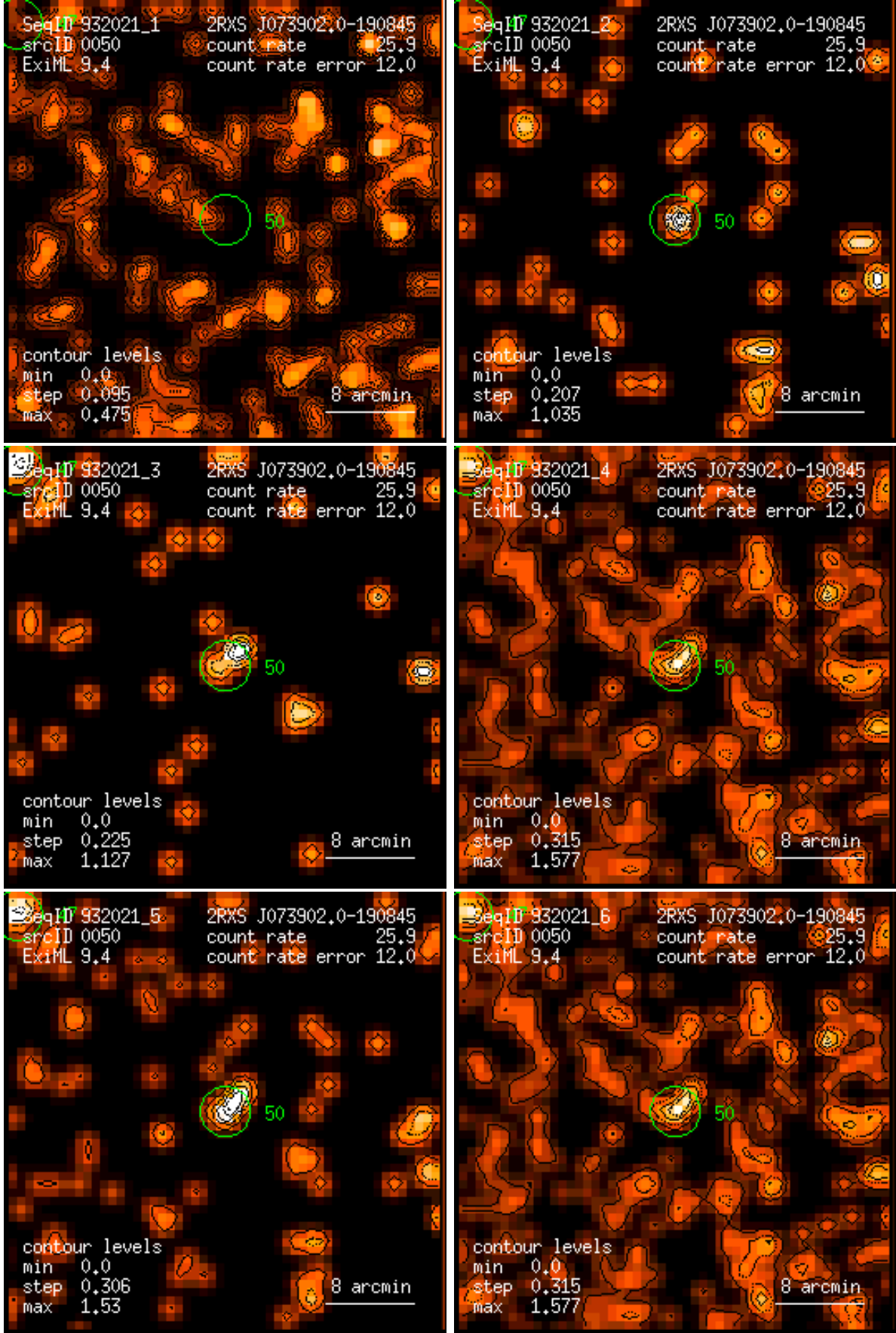
Figure 50: RASS 932021: detection 0050: band rate images, Gaussian filter: (1) PSPC channels 11 – 41, (2) 52 – 90, (3) 91 – 201, (4) 11 – 235, (5) 52 – 201, (6) 11 – 201. Broad band rates in counts/ks. Band rate contour levels in counts/ks/arcmin 2 .
