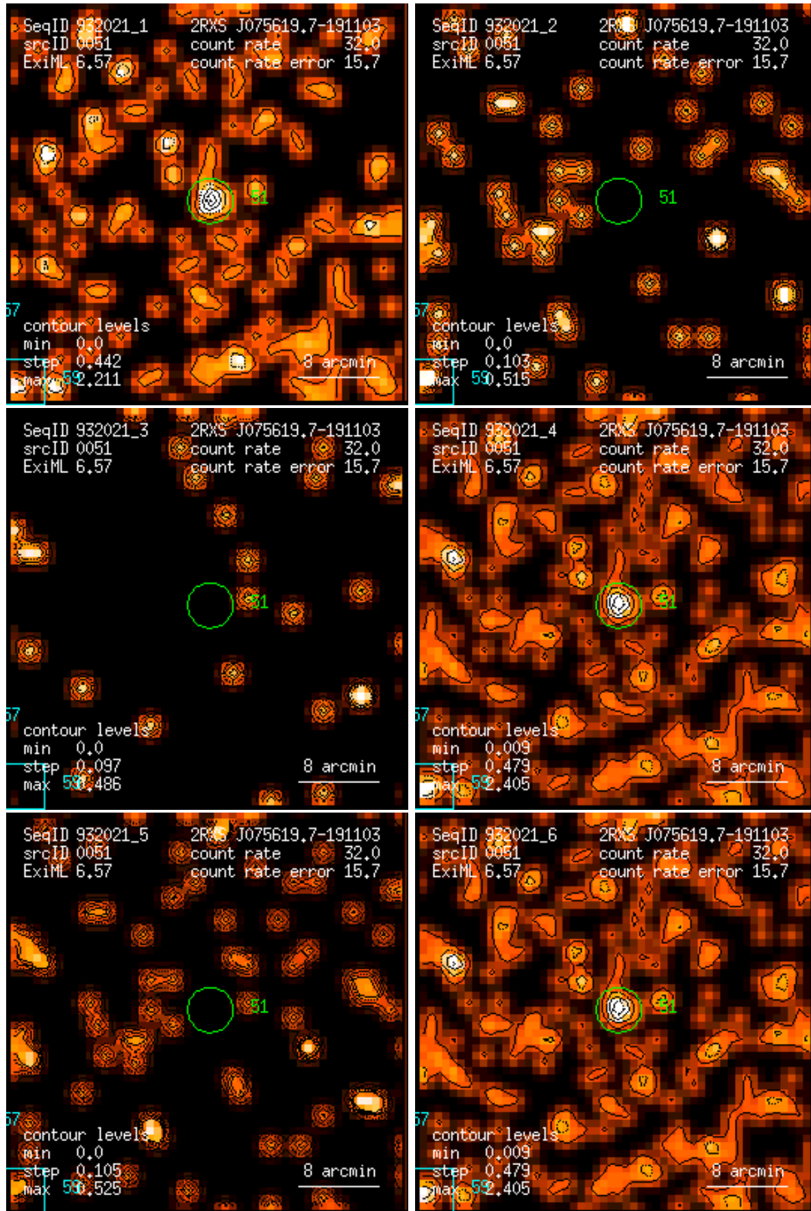
Figure 51: RASS 932021: detection 0051: band rate images, Gaussian filter: (1) PSPC channels 11 – 41, (2) 52 – 90, (3) 91 – 201, (4) 11 – 235, (5) 52 – 201, (6) 11 – 201. Broad band rates in counts/ks. Band rate contour levels in counts/ks/arcmin 2 .
