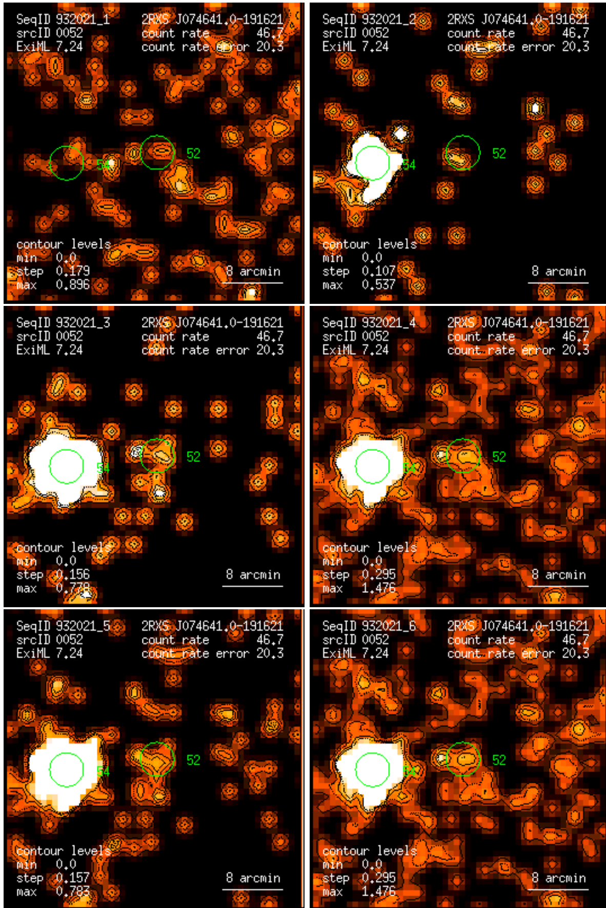
Figure 52: RASS 932021: detection 0052: band rate images, Gaussian filter: (1) PSPC channels 11 – 41, (2) 52 – 90, (3) 91 – 201, (4) 11 – 235, (5) 52 – 201, (6) 11 – 201. Broad band rates in counts/ks. Band rate contour levels in counts/ks/arcmin 2 .
