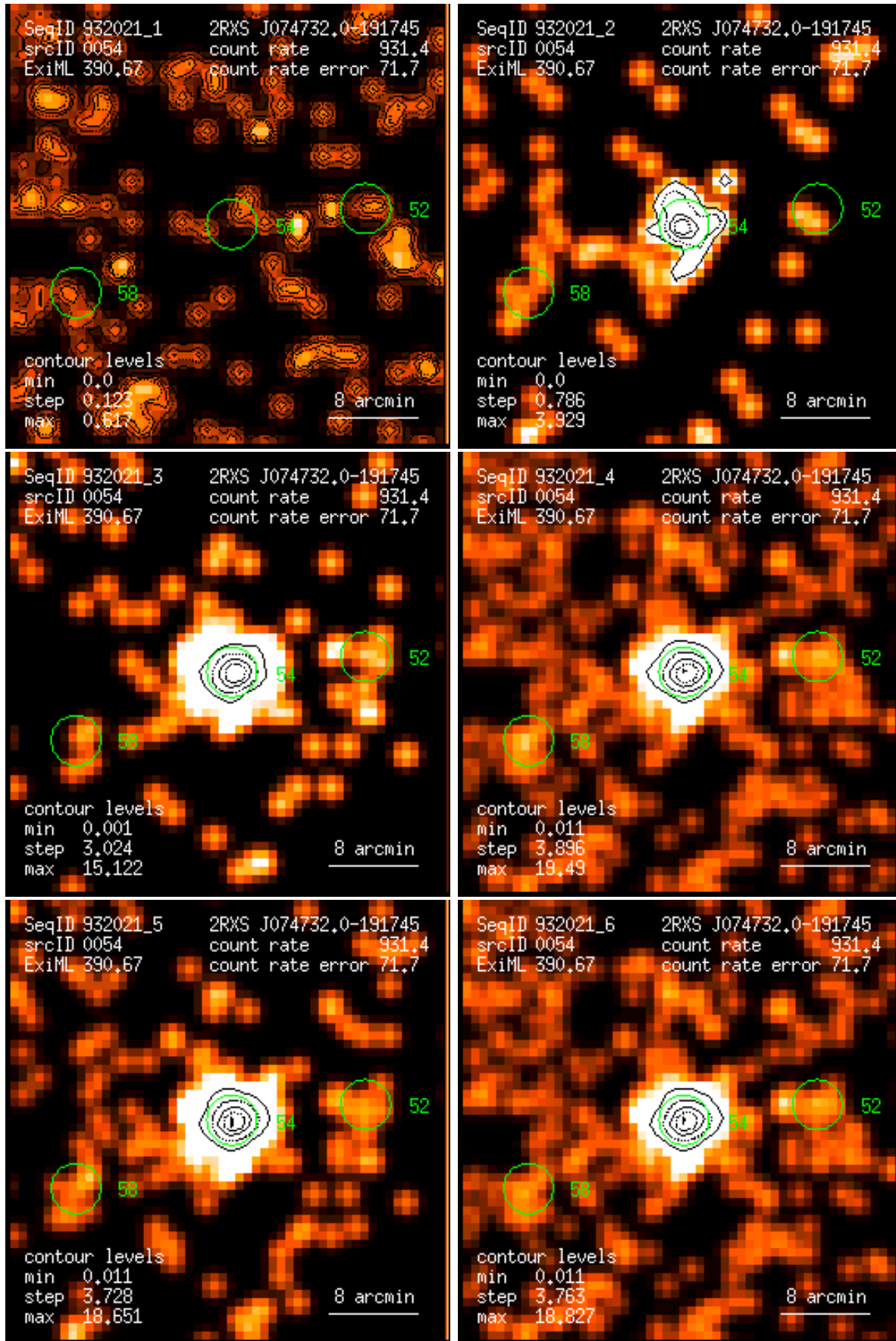
Figure 54: RASS 932021: detection 0054: band rate images, Gaussian filter: (1) PSPC channels 11 – 41, (2) 52 – 90, (3) 91 – 201, (4) 11 – 235, (5) 52 – 201, (6) 11 – 201. Broad band rates in counts/ks. Band rate contour levels in counts/ks/arcmin 2 .
