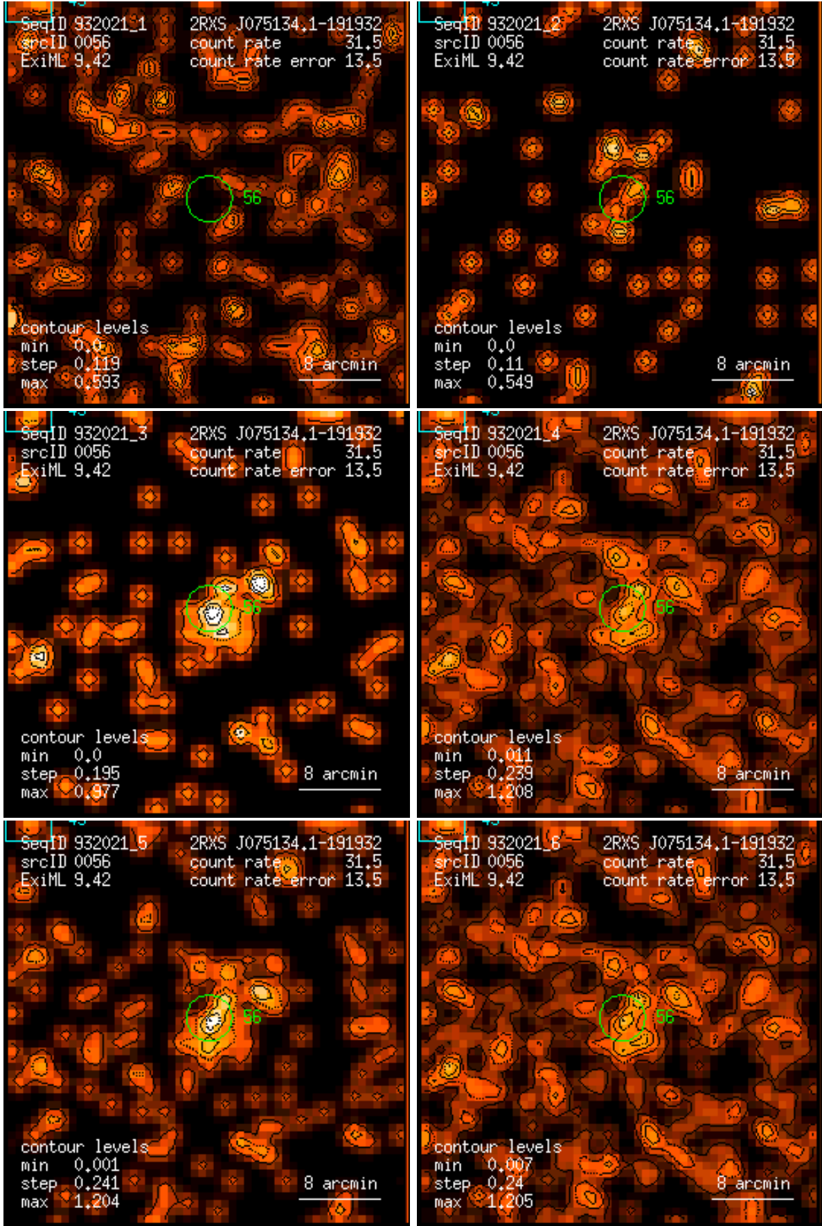
Figure 56: RASS 932021: detection 0056: band rate images, Gaussian filter: (1) PSPC channels 11 – 41, (2) 52 – 90, (3) 91 – 201, (4) 11 – 235, (5) 52 – 201, (6) 11 – 201. Broad band rates in counts/ks. Band rate contour levels in counts/ks/arcmin 2 .
