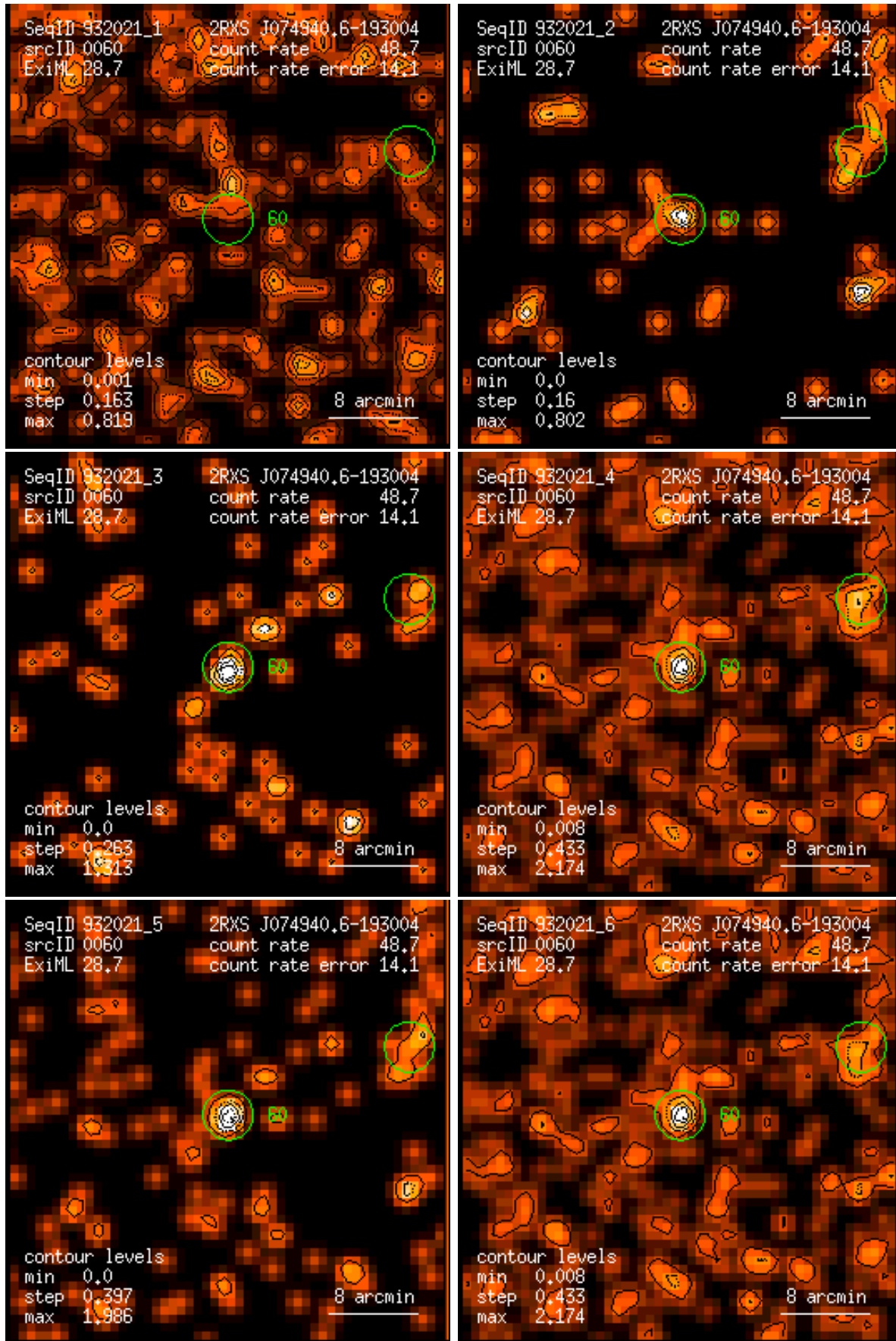
Figure 60: RASS 932021: detection 0060: band rate images, Gaussian filter: (1) PSPC channels 11 – 41, (2) 52 – 90, (3) 91 – 201, (4) 11 – 235, (5) 52 – 201, (6) 11 – 201. Broad band rates in counts/ks. Band rate contour levels in counts/ks/arcmin 2 .
