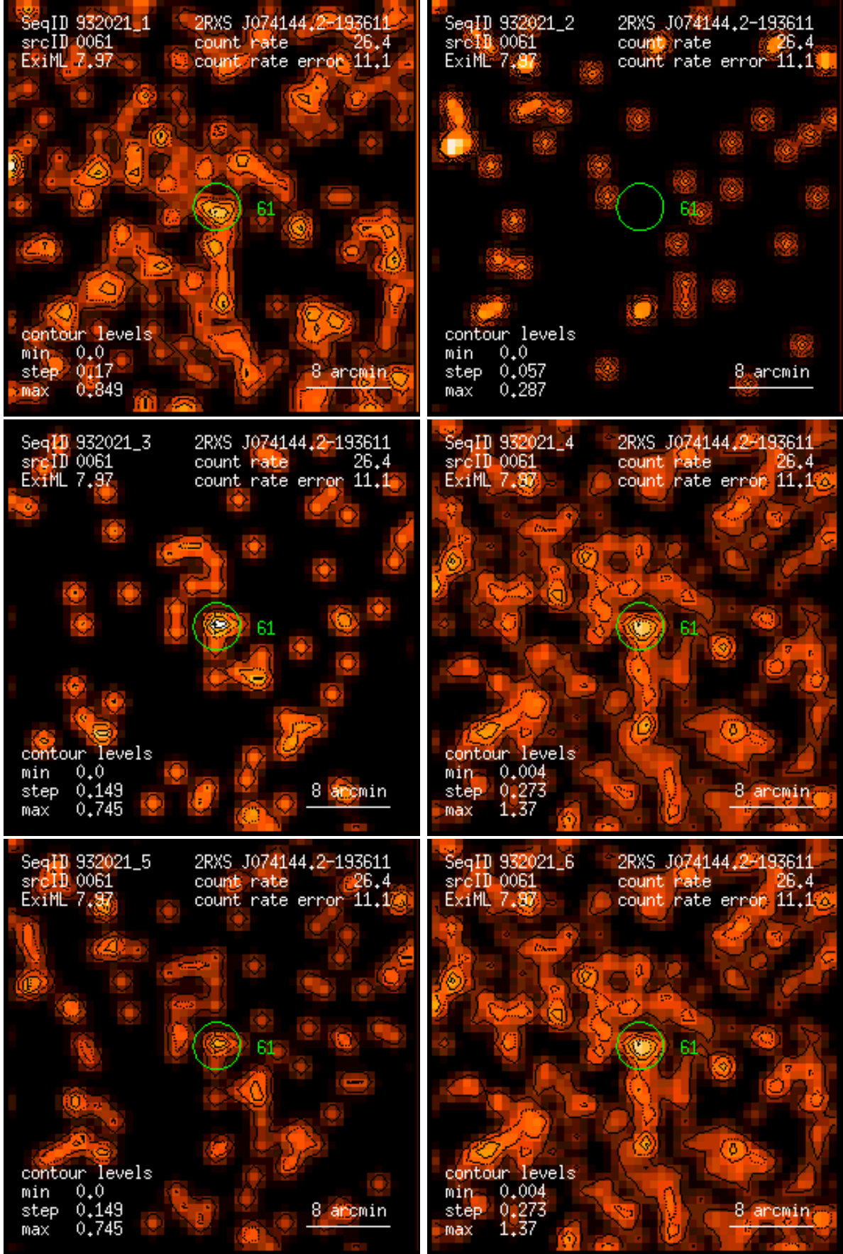
Figure 61: RASS 932021: detection 0061: band rate images, Gaussian filter: (1) PSPC channels 11 – 41, (2) 52 – 90, (3) 91 – 201, (4) 11 – 235, (5) 52 – 201, (6) 11 – 201. Broad band rates in counts/ks. Band rate contour levels in counts/ks/arcmin 2 .
