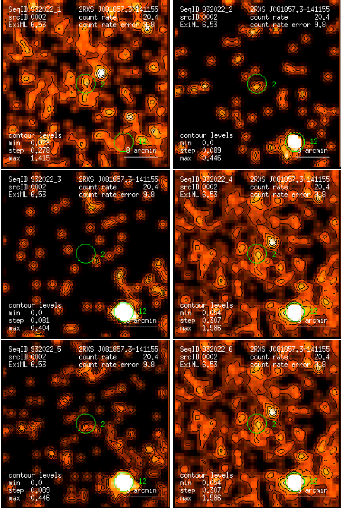
Figure 2: RASS 932022: detection 0002: band rate images, Gaussian filter: (1) PSPC channels 11 – 41, (2) 52 – 90, (3) 91 – 201, (4) 11 – 235, (5) 52 – 201, (6) 11 – 201. Broad band rates in counts/ks. Band rate contour levels in counts/ks/arcmin 2 .
