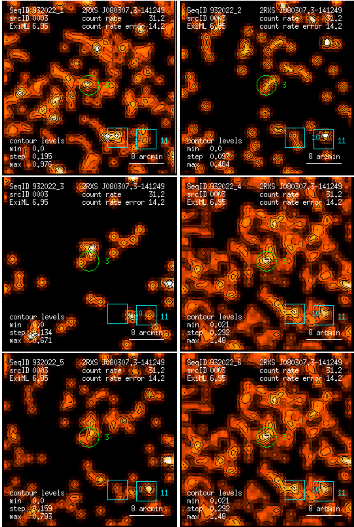
Figure 3: RASS 932022: detection 0003: band rate images, Gaussian filter: (1) PSPC channels 11 – 41, (2) 52 – 90, (3) 91 – 201, (4) 11 – 235, (5) 52 – 201, (6) 11 – 201. Broad band rates in counts/ks. Band rate contour levels in counts/ks/arcmin 2 .
