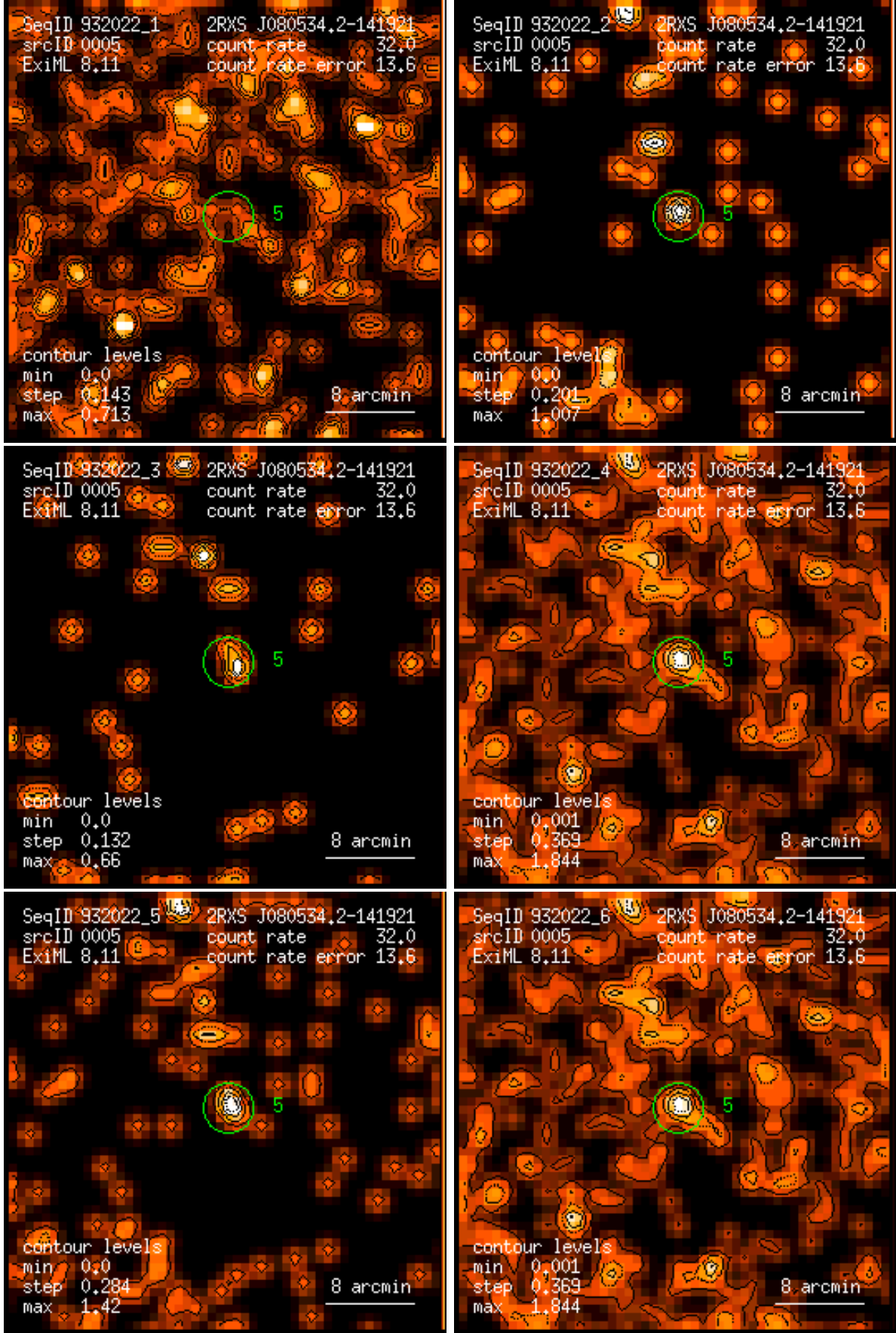
Figure 5: RASS 932022: detection 0005: band rate images, Gaussian filter: (1) PSPC channels 11 – 41, (2) 52 – 90, (3) 91 – 201, (4) 11 – 235, (5) 52 – 201, (6) 11 – 201. Broad band rates in counts/ks. Band rate contour levels in counts/ks/arcmin 2 .
