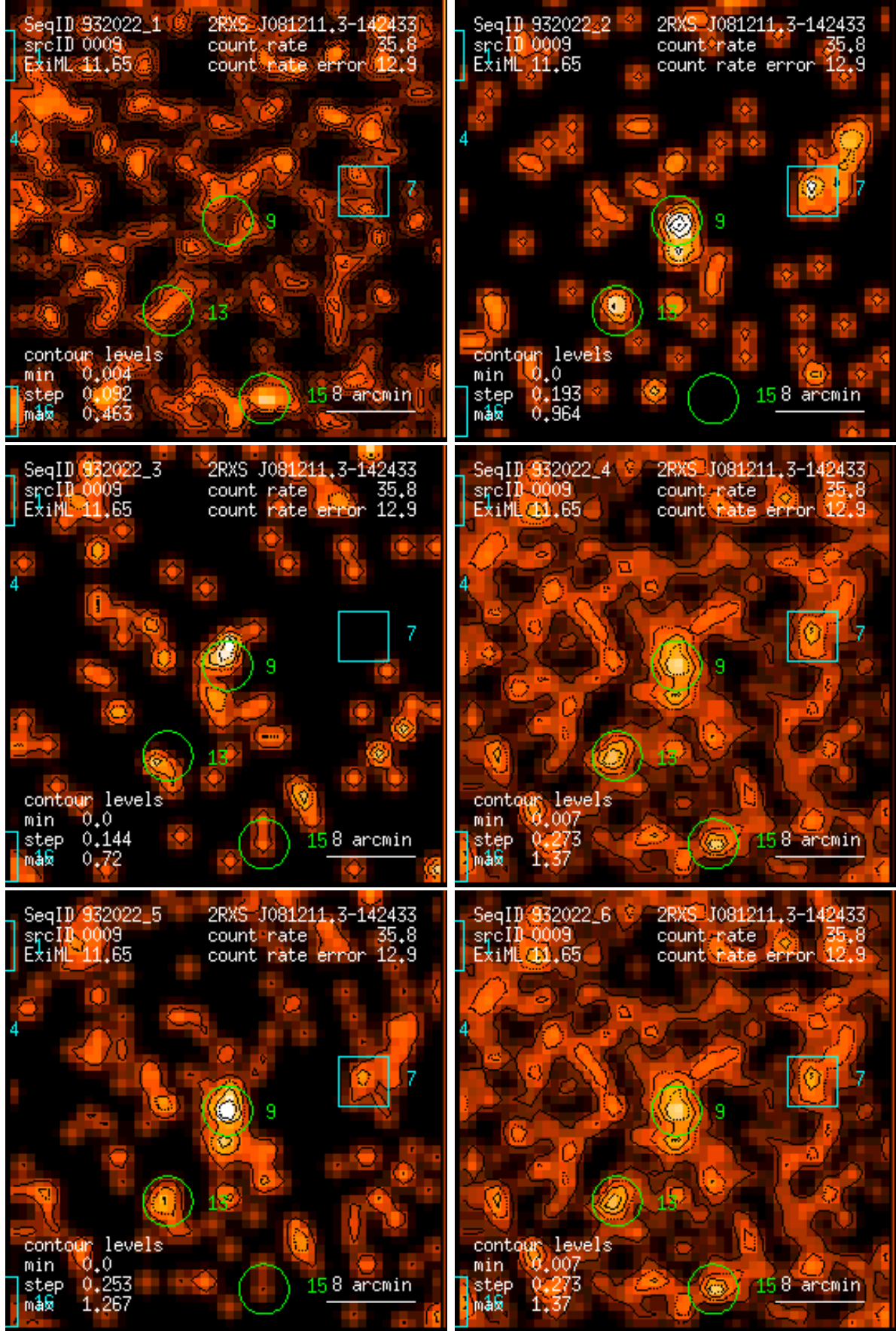
Figure 9: RASS 932022: detection 0009: band rate images, Gaussian filter: (1) PSPC channels 11 – 41, (2) 52 – 90, (3) 91 – 201, (4) 11 – 235, (5) 52 – 201, (6) 11 – 201. Broad band rates in counts/ks. Band rate contour levels in counts/ks/arcmin 2 .
