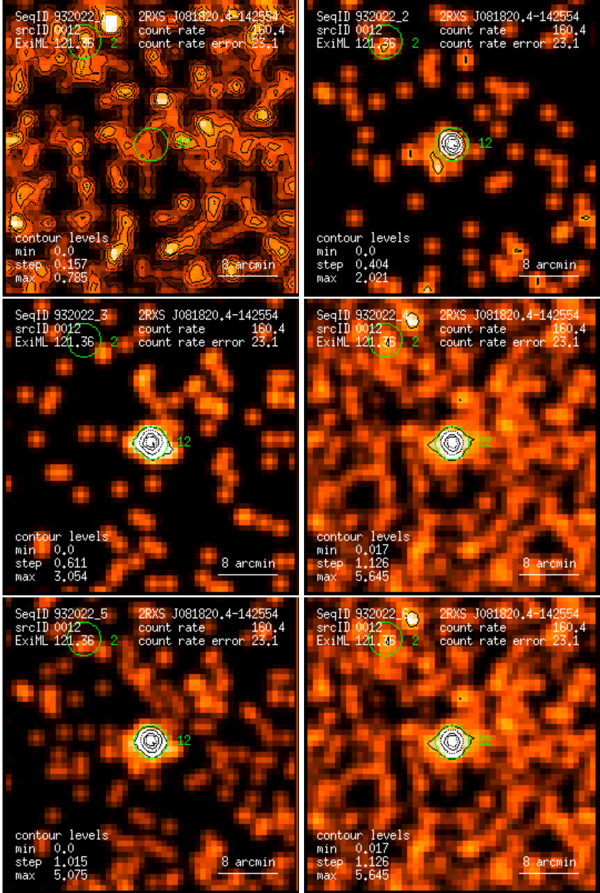
Figure 12: RASS 932022: detection 0012: band rate images, Gaussian filter: (1) PSPC channels 11 – 41, (2) 52 – 90, (3) 91 – 201, (4) 11 – 235, (5) 52 – 201, (6) 11 – 201. Broad band rates in counts/ks. Band rate contour levels in counts/ks/arcmin 2 .
