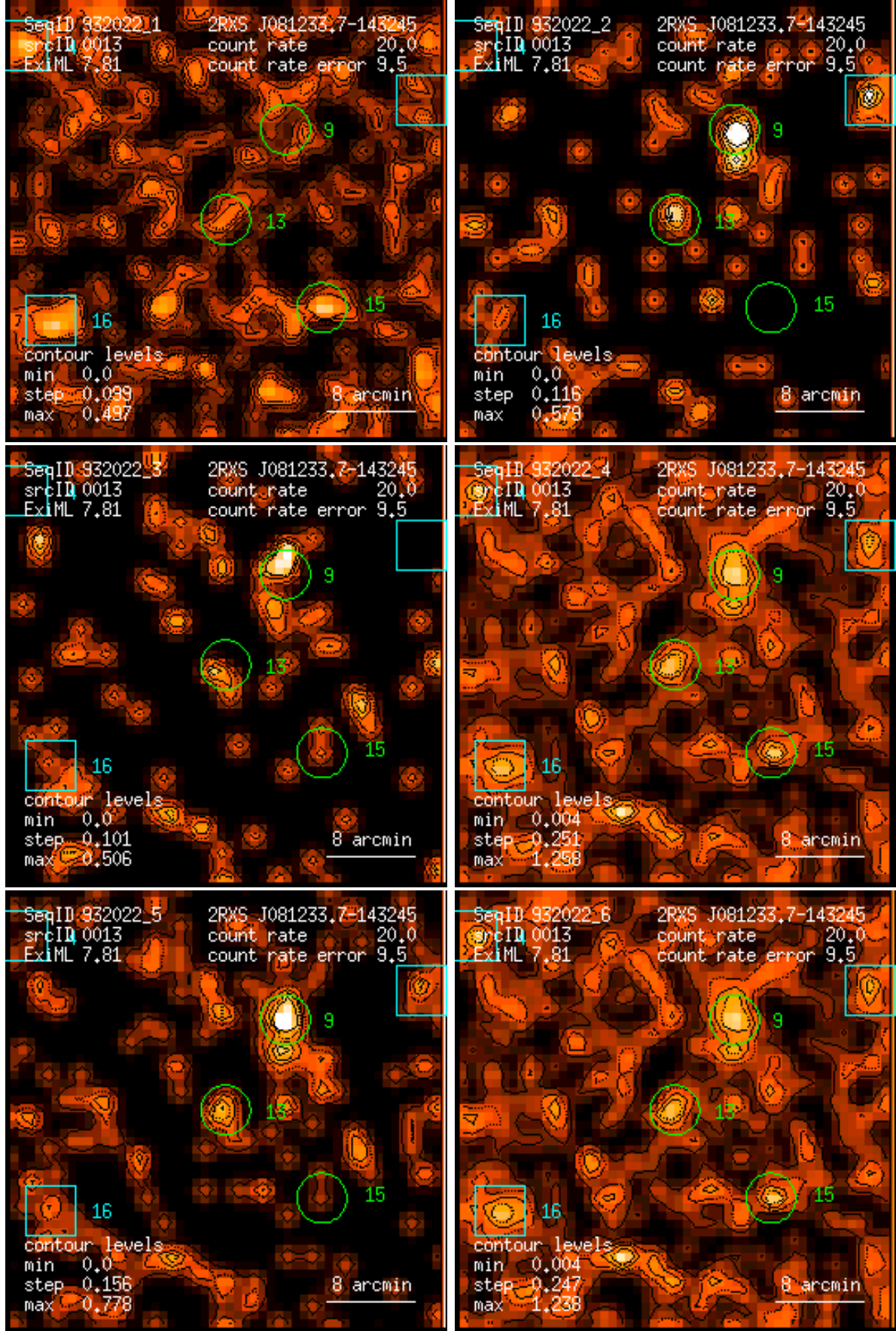
Figure 13: RASS 932022: detection 0013: band rate images, Gaussian filter: (1) PSPC channels 11 – 41, (2) 52 – 90, (3) 91 – 201, (4) 11 – 235, (5) 52 – 201, (6) 11 – 201. Broad band rates in counts/ks. Band rate contour levels in counts/ks/arcmin 2 .
