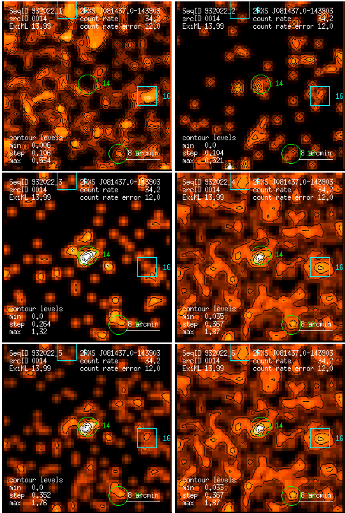
Figure 14: RASS 932022: detection 0014: band rate images, Gaussian filter: (1) PSPC channels 11 – 41, (2) 52 – 90, (3) 91 – 201, (4) 11 – 235, (5) 52 – 201, (6) 11 – 201. Broad band rates in counts/ks. Band rate contour levels in counts/ks/arcmin 2 .
