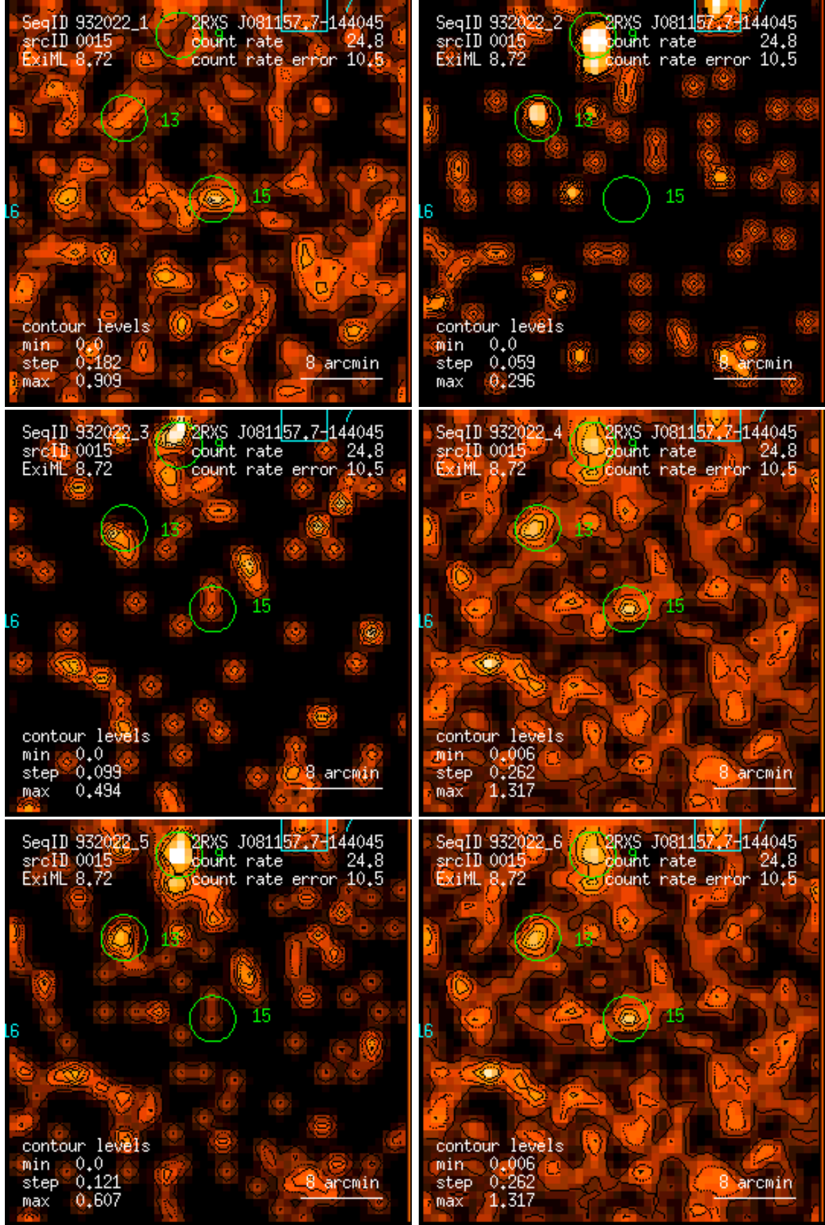
Figure 15: RASS 932022: detection 0015: band rate images, Gaussian filter: (1) PSPC channels 11 – 41, (2) 52 – 90, (3) 91 – 201, (4) 11 – 235, (5) 52 – 201, (6) 11 – 201. Broad band rates in counts/ks. Band rate contour levels in counts/ks/arcmin 2 .
