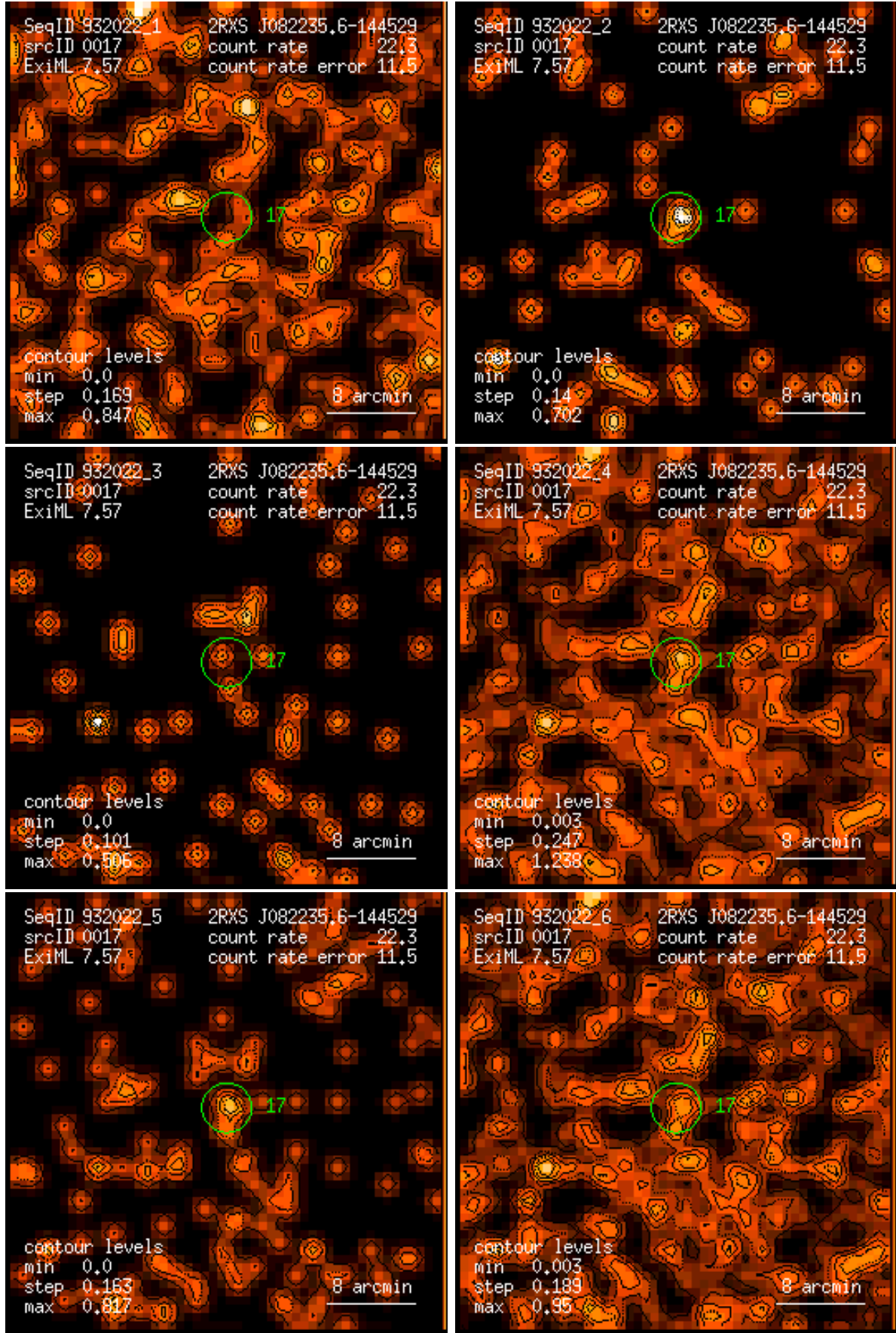
Figure 17: RASS 932022: detection 0017: band rate images, Gaussian filter: (1) PSPC channels 11 – 41, (2) 52 – 90, (3) 91 – 201, (4) 11 – 235, (5) 52 – 201, (6) 11 – 201. Broad band rates in counts/ks. Band rate contour levels in counts/ks/arcmin 2 .
