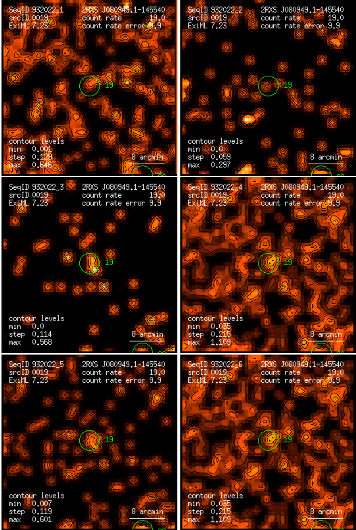
Figure 19: RASS 932022: detection 0019: band rate images, Gaussian filter: (1) PSPC channels 11 – 41, (2) 52 – 90, (3) 91 – 201, (4) 11 – 235, (5) 52 – 201, (6) 11 – 201. Broad band rates in counts/ks. Band rate contour levels in counts/ks/arcmin 2 .
