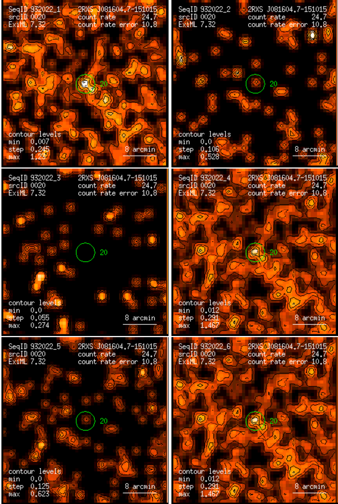
Figure 20: RASS 932022: detection 0020: band rate images, Gaussian filter: (1) PSPC channels 11 – 41, (2) 52 – 90, (3) 91 – 201, (4) 11 – 235, (5) 52 – 201, (6) 11 – 201. Broad band rates in counts/ks. Band rate contour levels in counts/ks/arcmin 2 .
