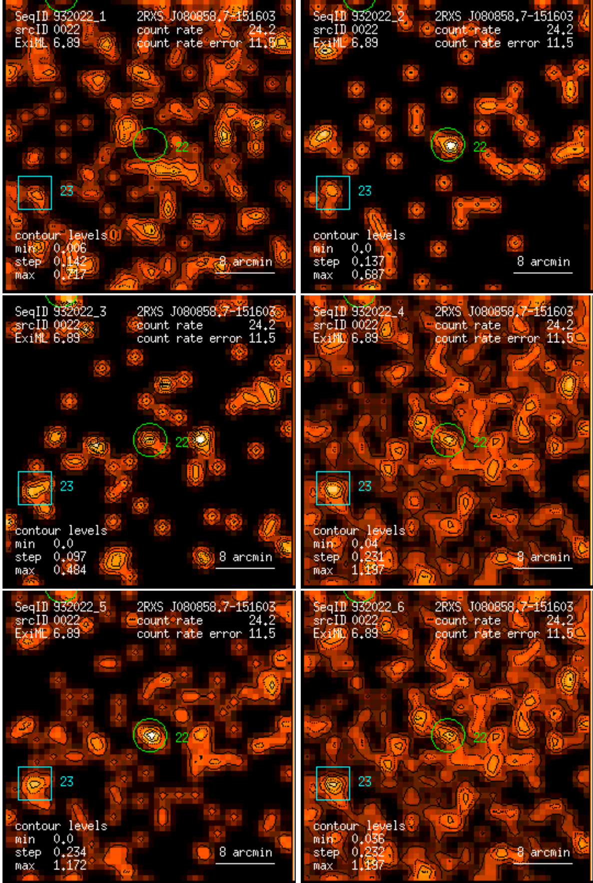
Figure 22: RASS 932022: detection 0022: band rate images, Gaussian filter: (1) PSPC channels 11 – 41, (2) 52 – 90, (3) 91 – 201, (4) 11 – 235, (5) 52 – 201, (6) 11 – 201. Broad band rates in counts/ks. Band rate contour levels in counts/ks/arcmin 2 .
