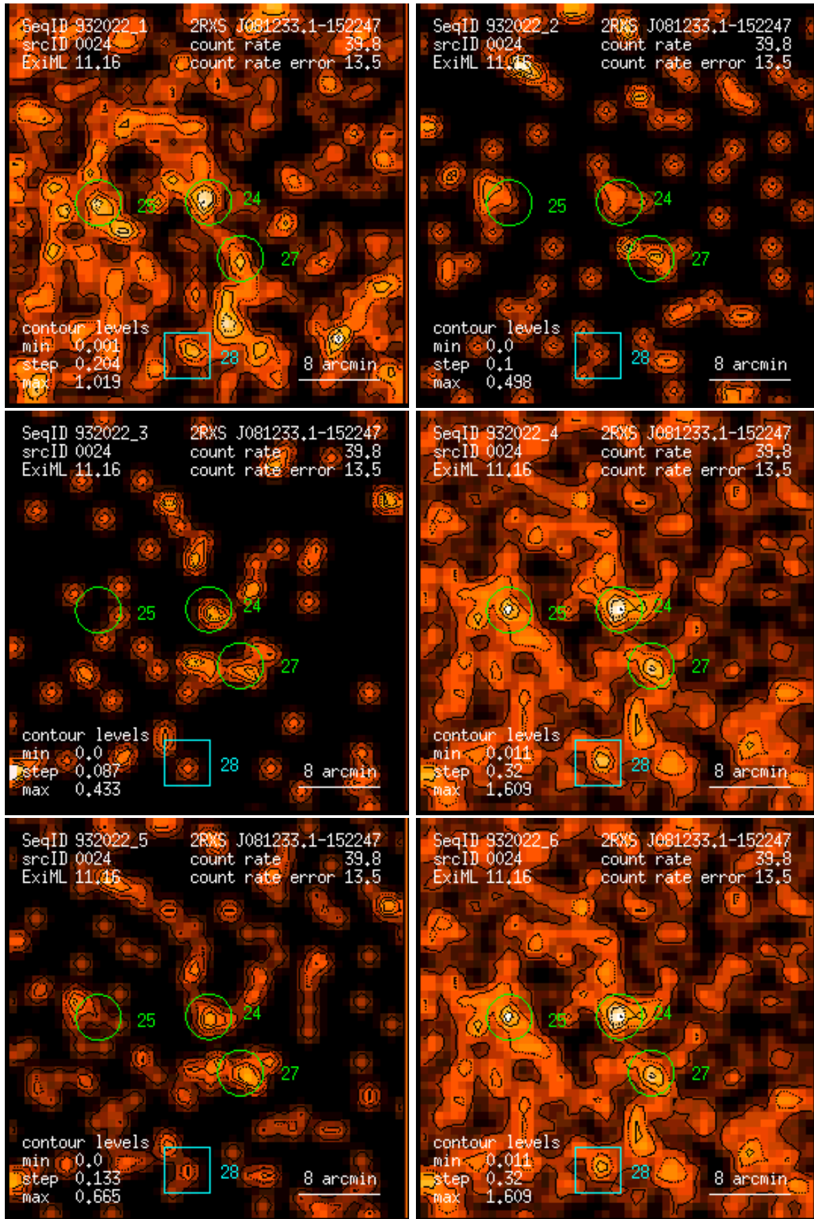
Figure 24: RASS 932022: detection 0024: band rate images, Gaussian filter: (1) PSPC channels 11 – 41, (2) 52 – 90, (3) 91 – 201, (4) 11 – 235, (5) 52 – 201, (6) 11 – 201. Broad band rates in counts/ks. Band rate contour levels in counts/ks/arcmin 2 .
