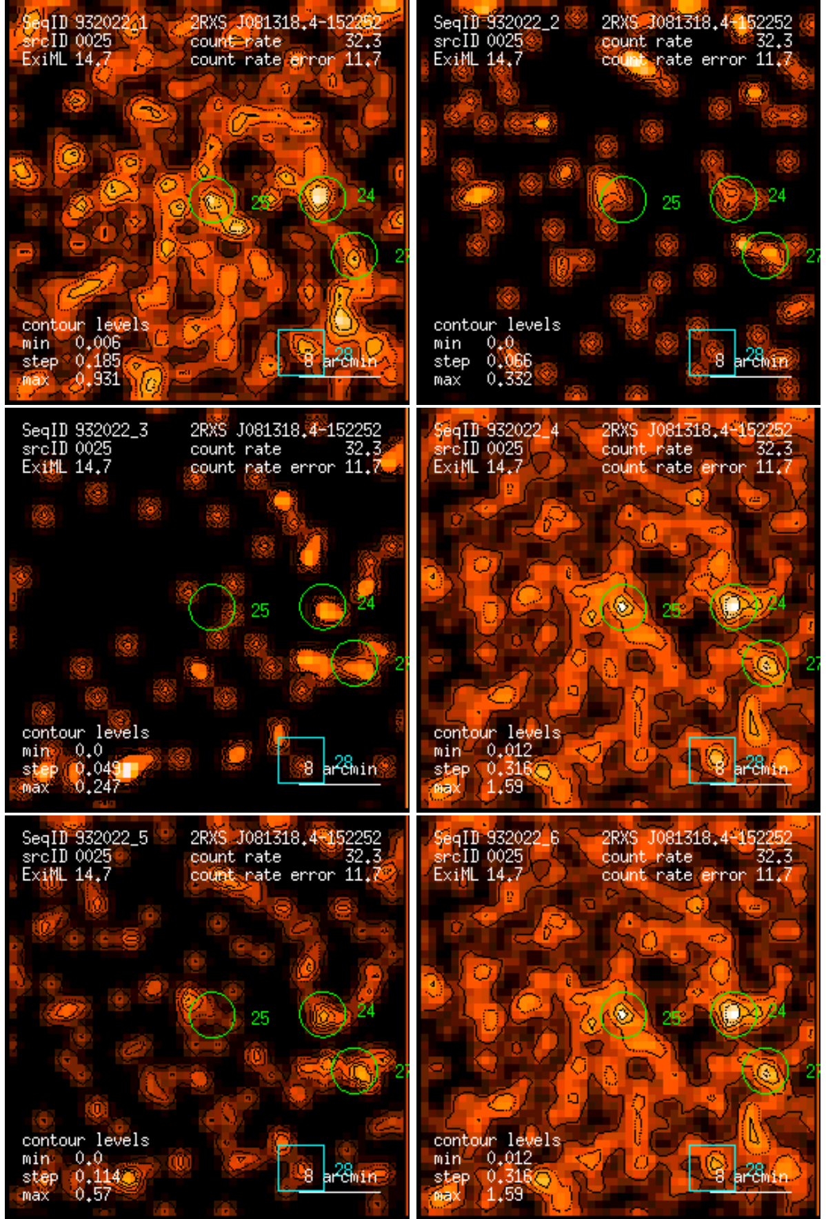
Figure 25: RASS 932022: detection 0025: band rate images, Gaussian filter: (1) PSPC channels 11 – 41, (2) 52 – 90, (3) 91 – 201, (4) 11 – 235, (5) 52 – 201, (6) 11 – 201. Broad band rates in counts/ks. Band rate contour levels in counts/ks/arcmin 2 .
