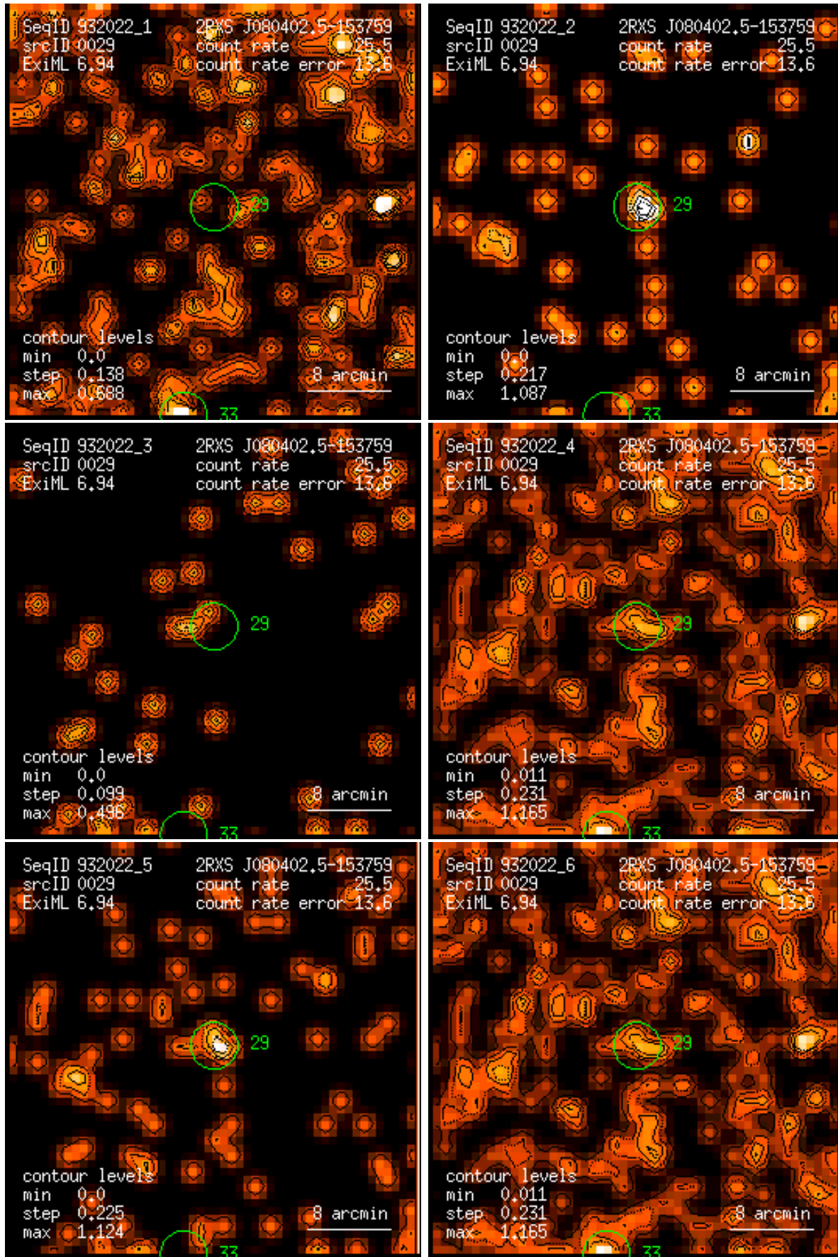
Figure 29: RASS 932022: detection 0029: band rate images, Gaussian filter: (1) PSPC channels 11 – 41, (2) 52 – 90, (3) 91 – 201, (4) 11 – 235, (5) 52 – 201, (6) 11 – 201. Broad band rates in counts/ks. Band rate contour levels in counts/ks/arcmin 2 .
