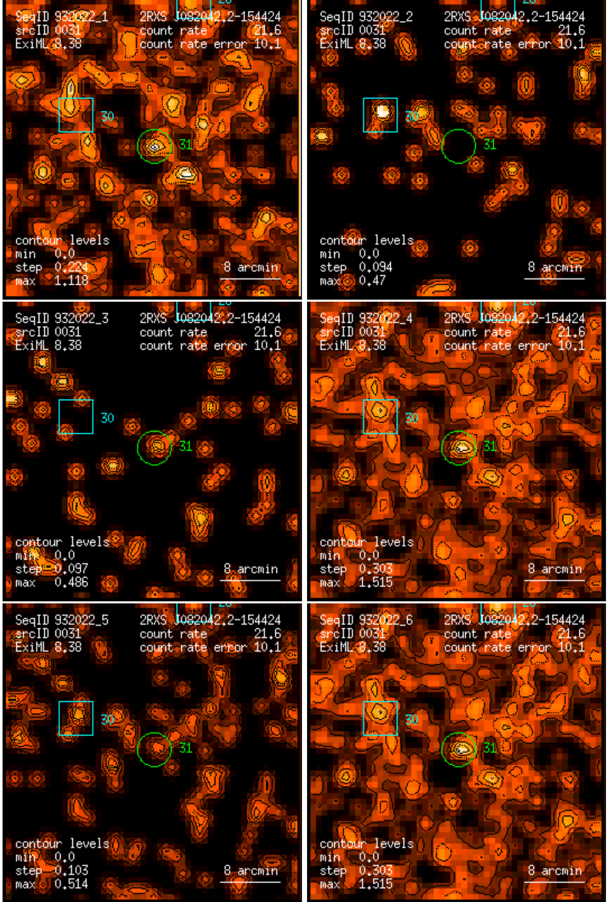
Figure 31: RASS 932022: detection 0031: band rate images, Gaussian filter: (1) PSPC channels 11 – 41, (2) 52 – 90, (3) 91 – 201, (4) 11 – 235, (5) 52 – 201, (6) 11 – 201. Broad band rates in counts/ks. Band rate contour levels in counts/ks/arcmin 2 .
