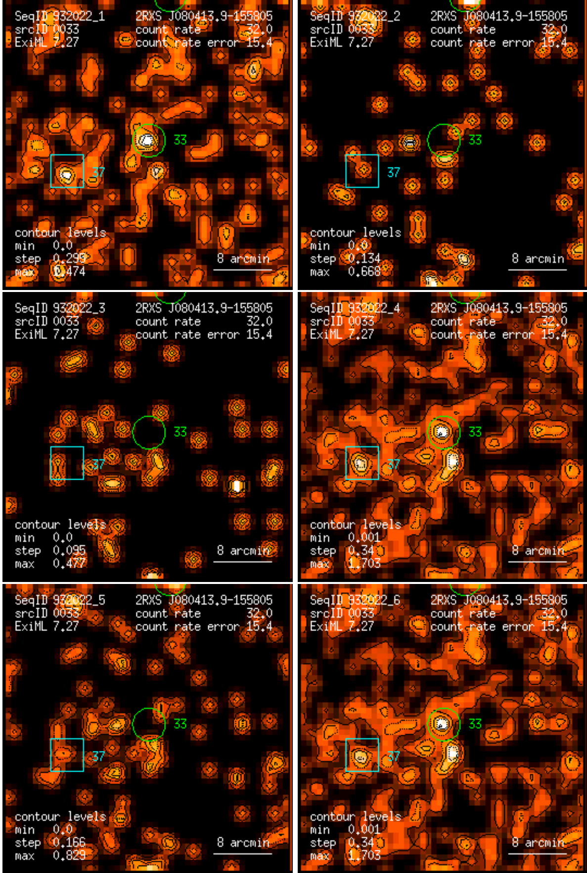
Figure 33: RASS 932022: detection 0033: band rate images, Gaussian filter: (1) PSPC channels 11 – 41, (2) 52 – 90, (3) 91 – 201, (4) 11 – 235, (5) 52 – 201, (6) 11 – 201. Broad band rates in counts/ks. Band rate contour levels in counts/ks/arcmin 2 .
