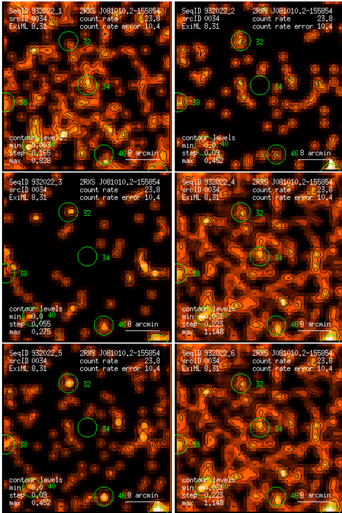
Figure 34: RASS 932022: detection 0034: band rate images, Gaussian filter: (1) PSPC channels 11 – 41, (2) 52 – 90, (3) 91 – 201, (4) 11 – 235, (5) 52 – 201, (6) 11 – 201. Broad band rates in counts/ks. Band rate contour levels in counts/ks/arcmin 2 .
