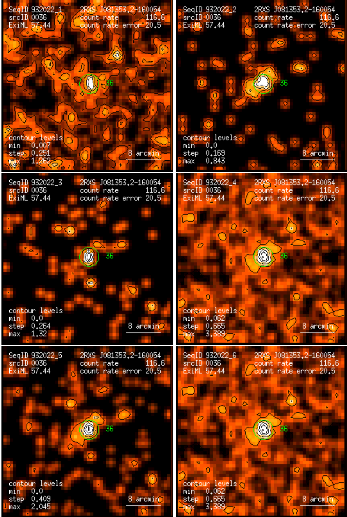
Figure 36: RASS 932022: detection 0036: band rate images, Gaussian filter: (1) PSPC channels 11 – 41, (2) 52 – 90, (3) 91 – 201, (4) 11 – 235, (5) 52 – 201, (6) 11 – 201. Broad band rates in counts/ks. Band rate contour levels in counts/ks/arcmin 2 .
