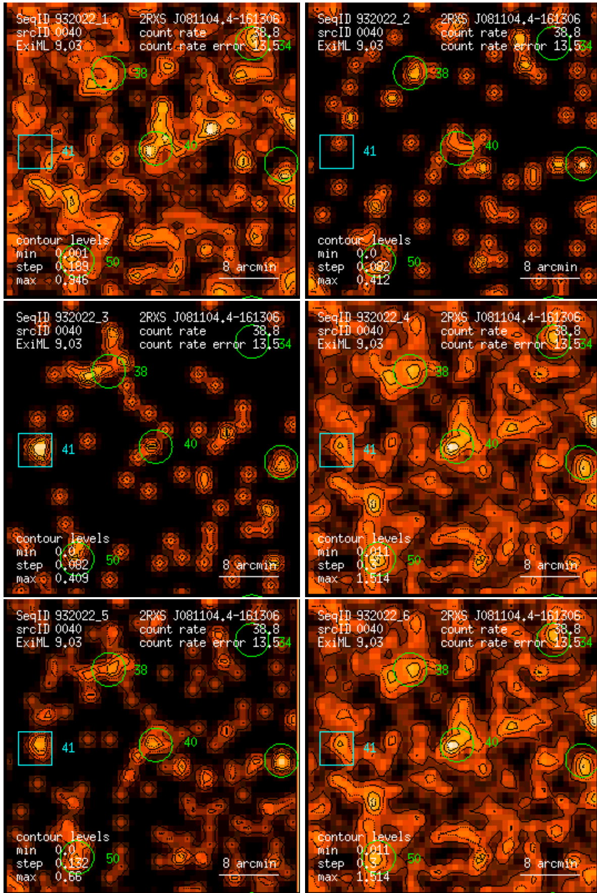
Figure 40: RASS 932022: detection 0040: band rate images, Gaussian filter: (1) PSPC channels 11 – 41, (2) 52 – 90, (3) 91 – 201, (4) 11 – 235, (5) 52 – 201, (6) 11 – 201. Broad band rates in counts/ks. Band rate contour levels in counts/ks/arcmin 2 .
