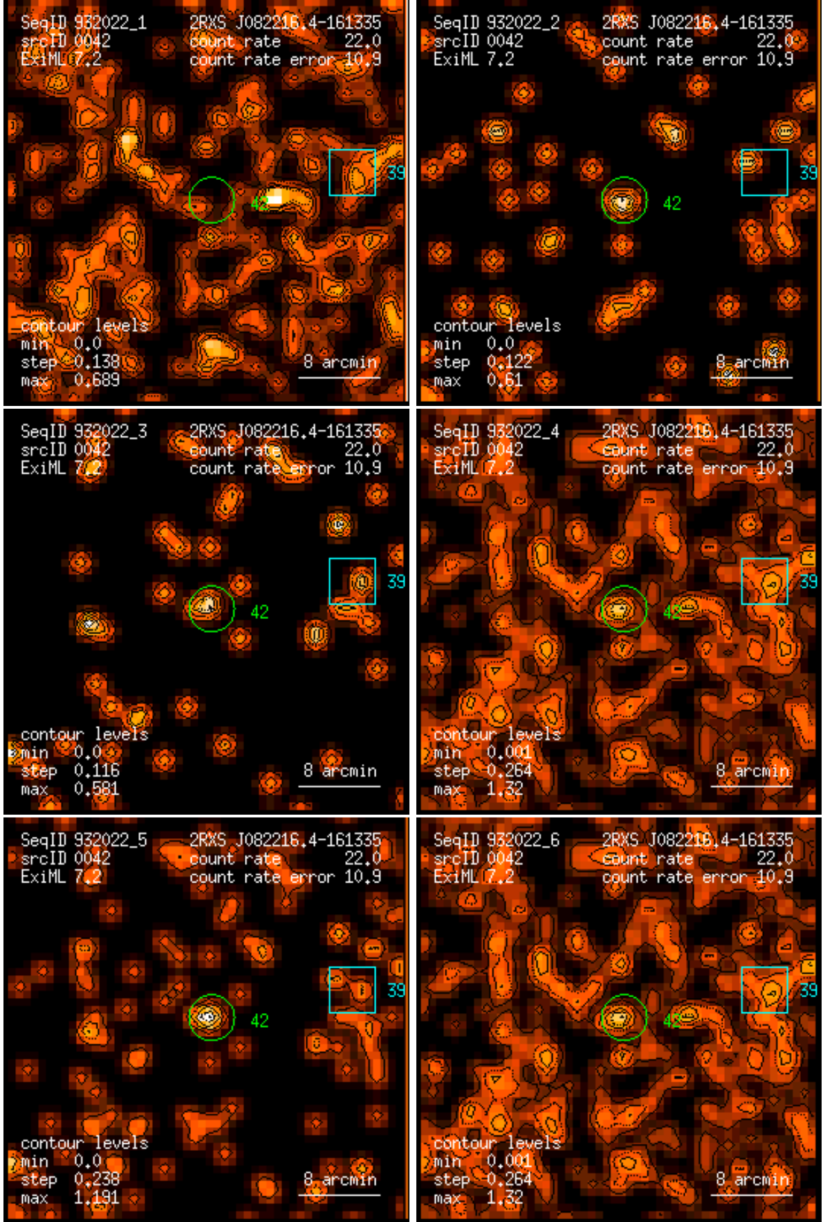
Figure 42: RASS 932022: detection 0042: band rate images, Gaussian filter: (1) PSPC channels 11 – 41, (2) 52 – 90, (3) 91 – 201, (4) 11 – 235, (5) 52 – 201, (6) 11 – 201. Broad band rates in counts/ks. Band rate contour levels in counts/ks/arcmin 2 .
