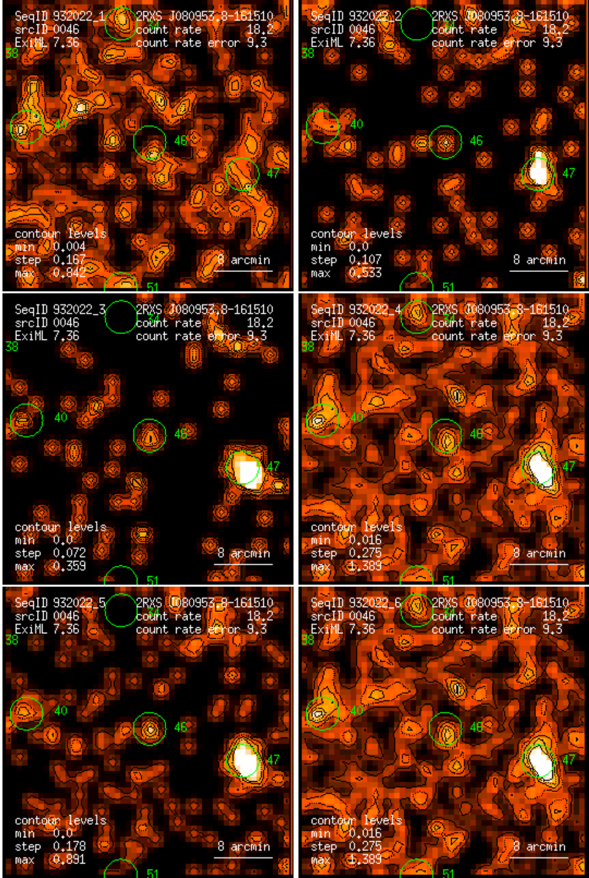
Figure 46: RASS 932022: detection 0046: band rate images, Gaussian filter: (1) PSPC channels 11 – 41, (2) 52 – 90, (3) 91 – 201, (4) 11 – 235, (5) 52 – 201, (6) 11 – 201. Broad band rates in counts/ks. Band rate contour levels in counts/ks/arcmin 2 .
