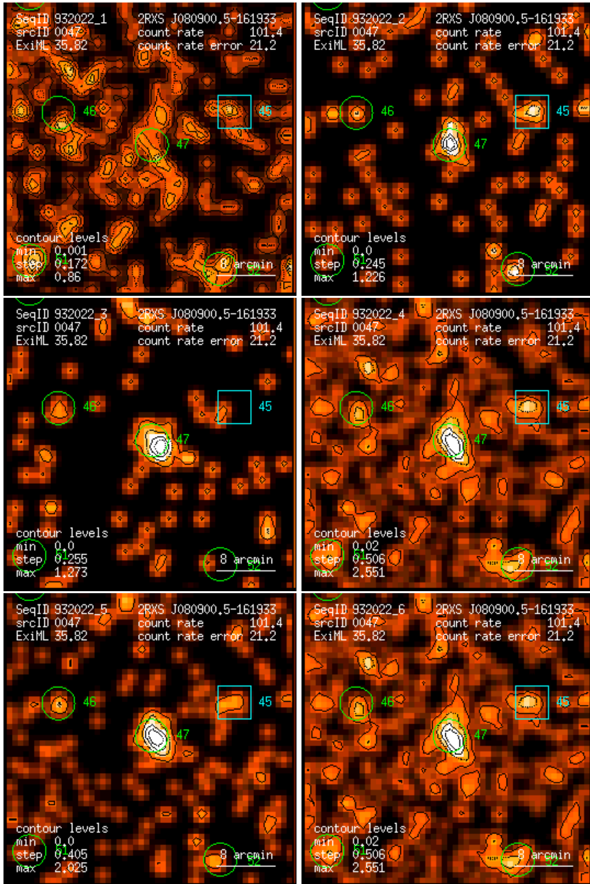
Figure 47: RASS 932022: detection 0047: band rate images, Gaussian filter: (1) PSPC channels 11 – 41, (2) 52 – 90, (3) 91 – 201, (4) 11 – 235, (5) 52 – 201, (6) 11 – 201. Broad band rates in counts/ks. Band rate contour levels in counts/ks/arcmin 2 .
