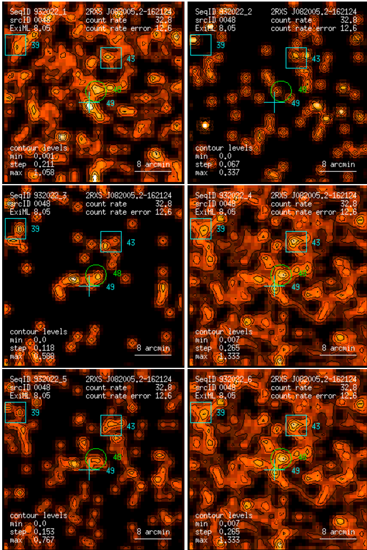
Figure 48: RASS 932022: detection 0048: band rate images, Gaussian filter: (1) PSPC channels 11 – 41, (2) 52 – 90, (3) 91 – 201, (4) 11 – 235, (5) 52 – 201, (6) 11 – 201. Broad band rates in counts/ks. Band rate contour levels in counts/ks/arcmin 2 .
