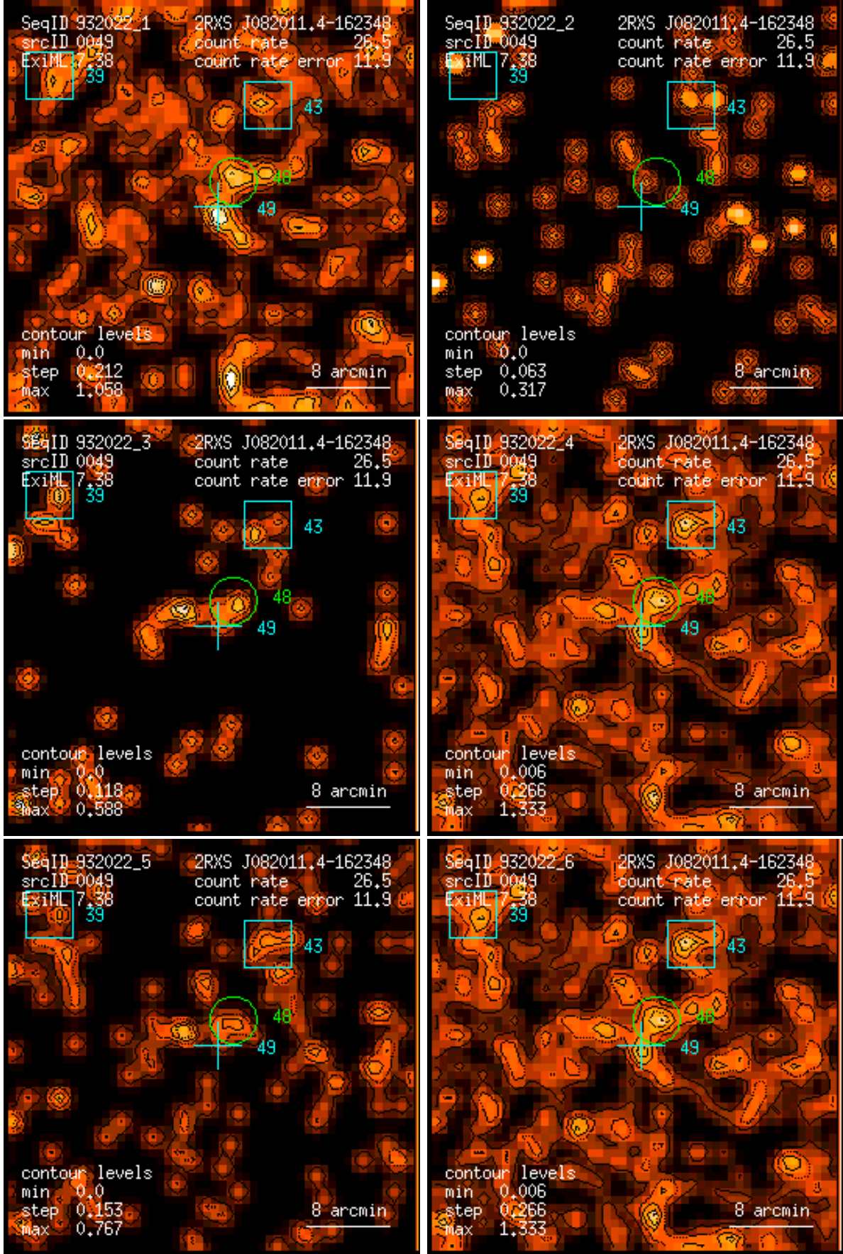
Figure 49: RASS 932022: detection 0049: band rate images, Gaussian filter: (1) PSPC channels 11 – 41, (2) 52 – 90, (3) 91 – 201, (4) 11 – 235, (5) 52 – 201, (6) 11 – 201. Broad band rates in counts/ks. Band rate contour levels in counts/ks/arcmin 2 .
