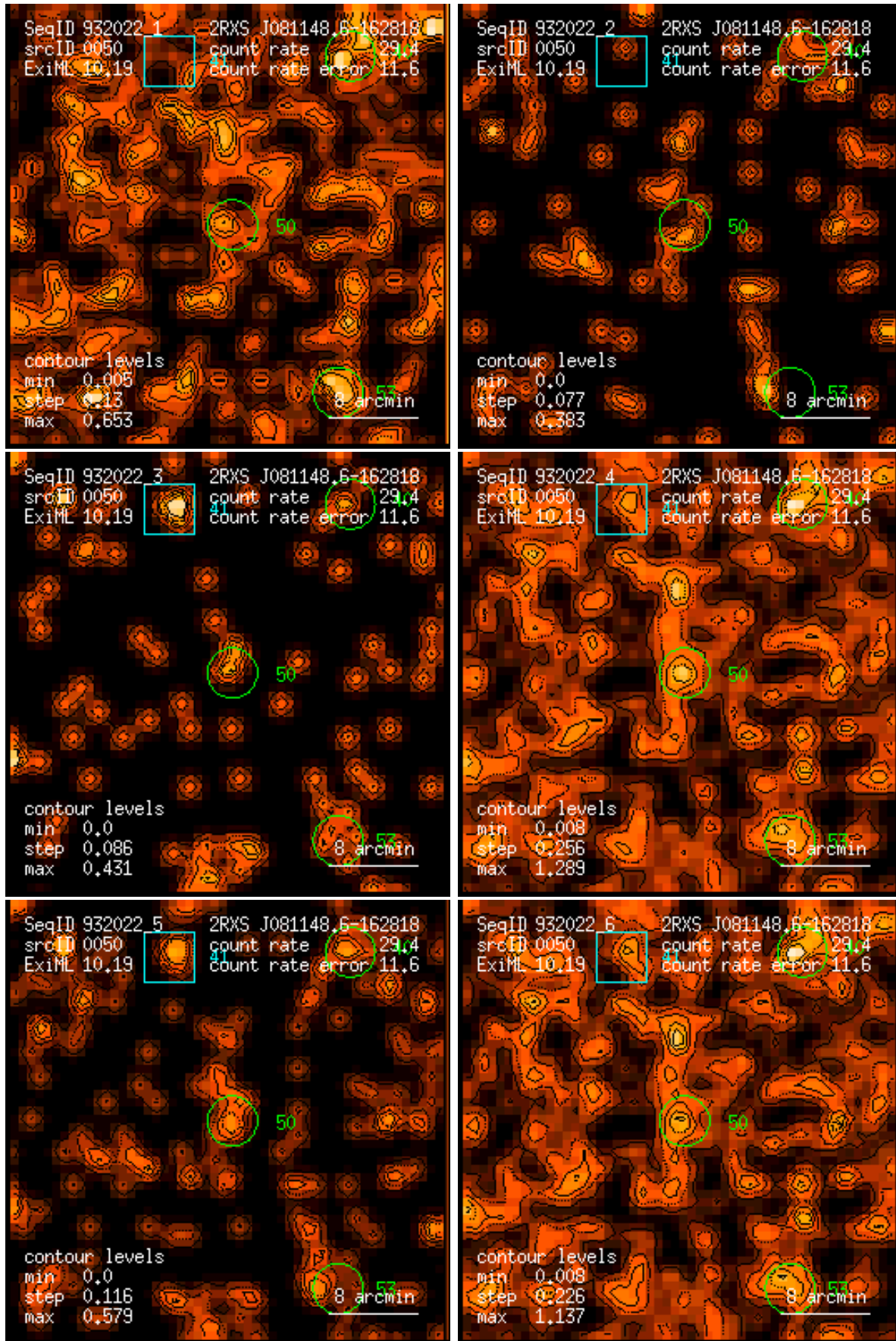
Figure 50: RASS 932022: detection 0050: band rate images, Gaussian filter: (1) PSPC channels 11 – 41, (2) 52 – 90, (3) 91 – 201, (4) 11 – 235, (5) 52 – 201, (6) 11 – 201. Broad band rates in counts/ks. Band rate contour levels in counts/ks/arcmin 2 .
